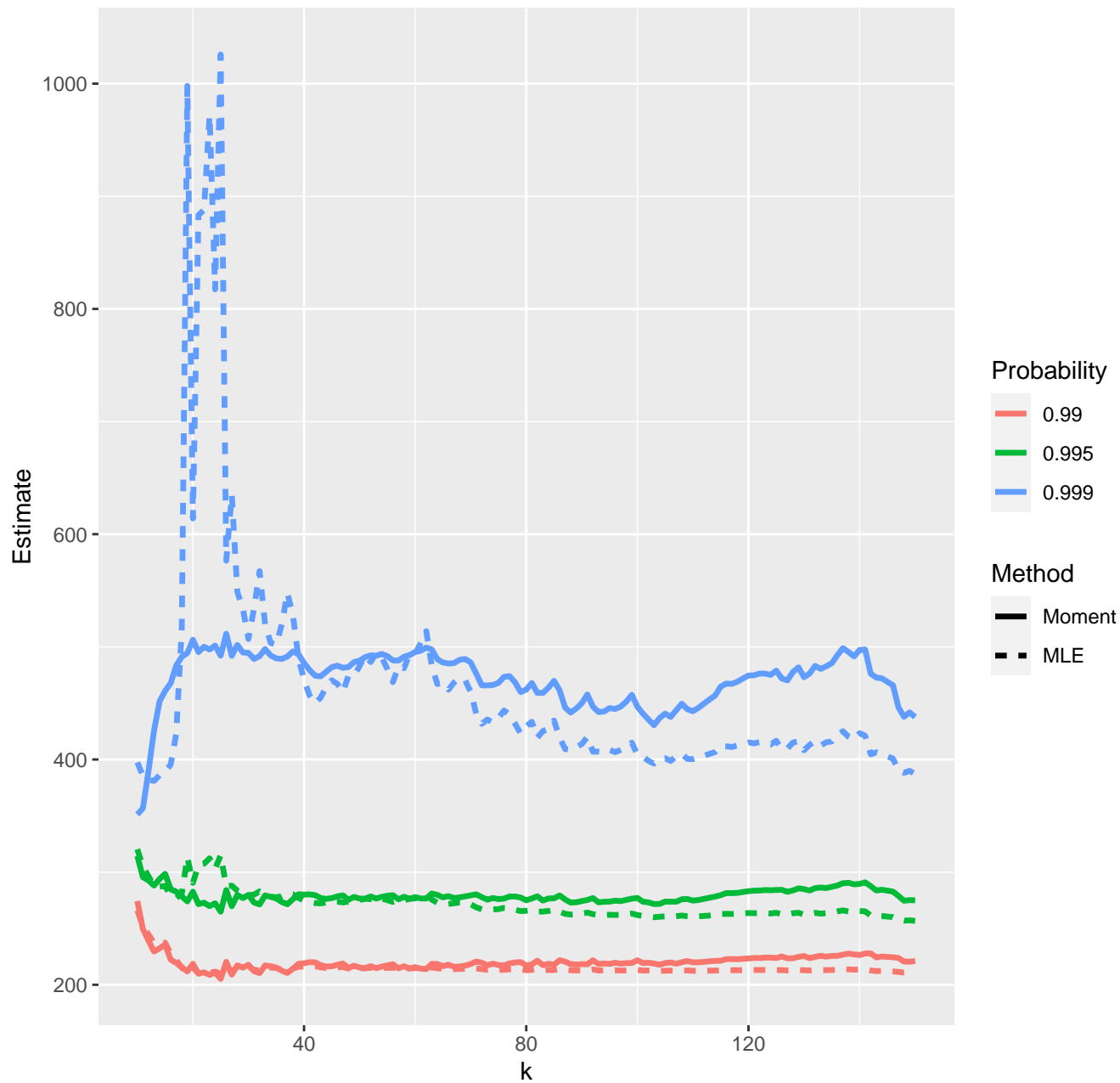
Estimates of high quantiles--26-03-2020
