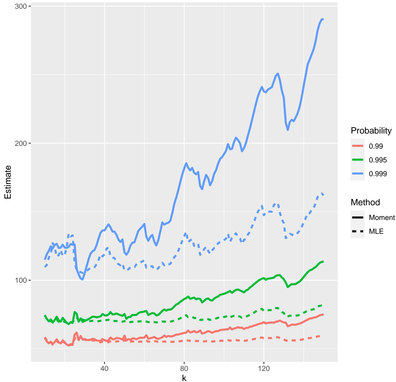
Estimates of high quantiles--15-03-2020
