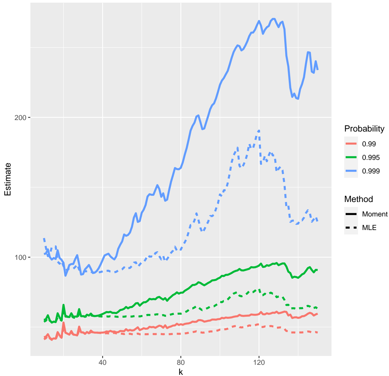
Estimates of high quantiles--13-03-2020
