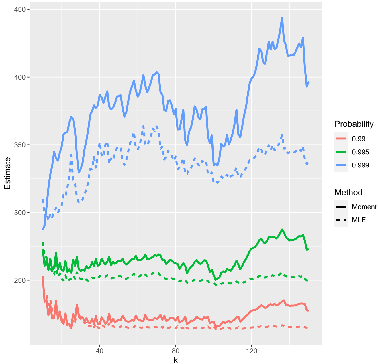
Estimates of high quantiles--10-04-2020
