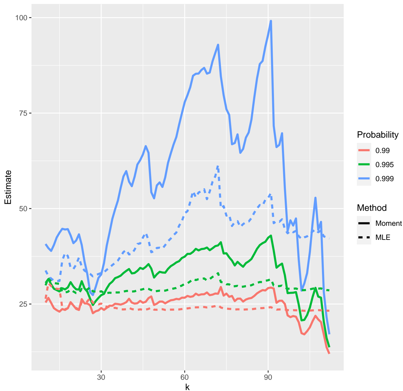
Estimates of high quantiles--10-03-2020
