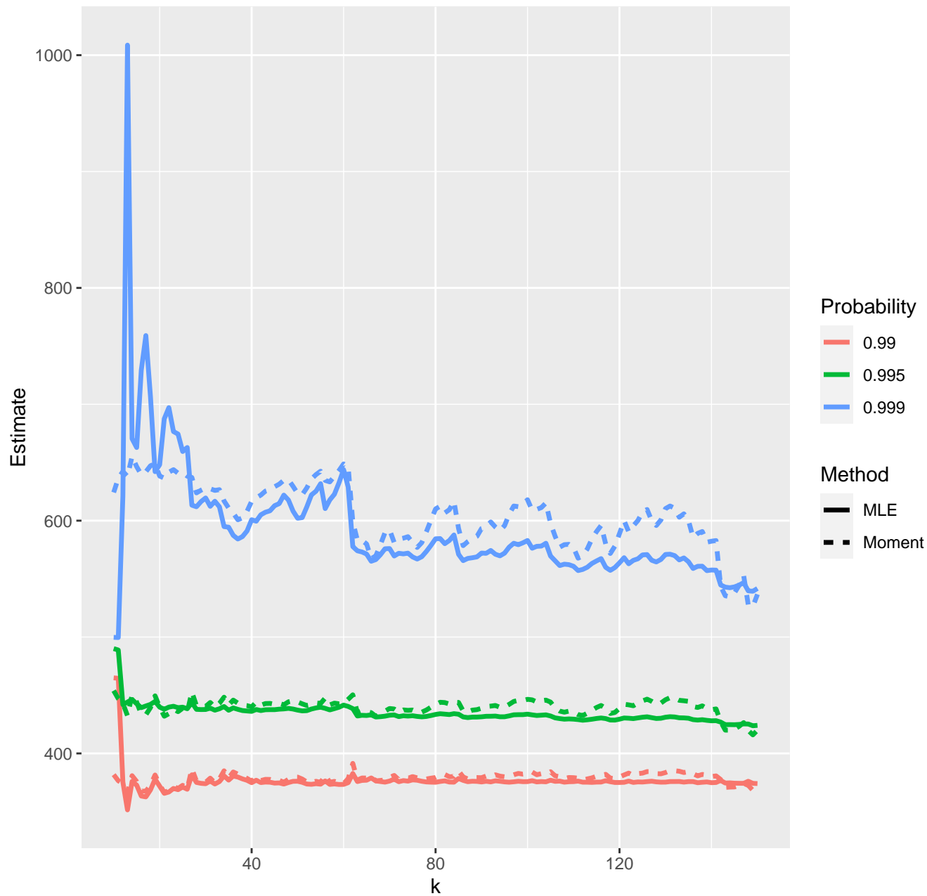
Estimates of high quantiles--28-09-2021
