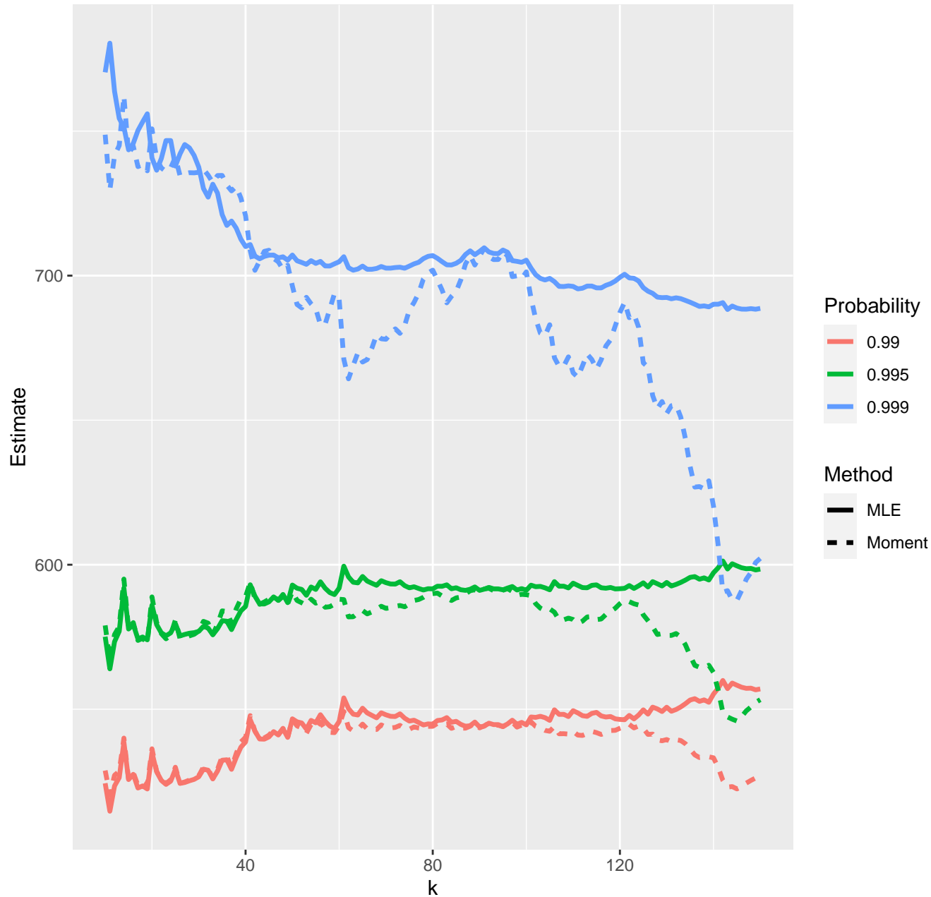
Estimates of high quantiles--28-06-2022
