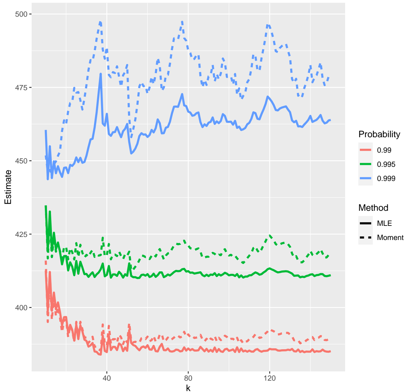
Estimates of high quantiles--25-10-2022
