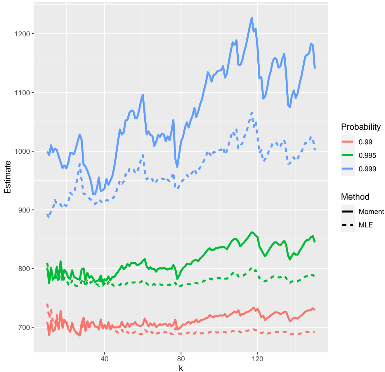
Estimates of high quantiles--24-04-2020
