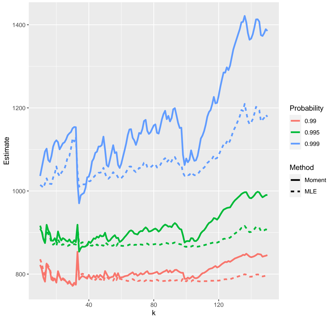
Estimates of high quantiles--23-05-2020
