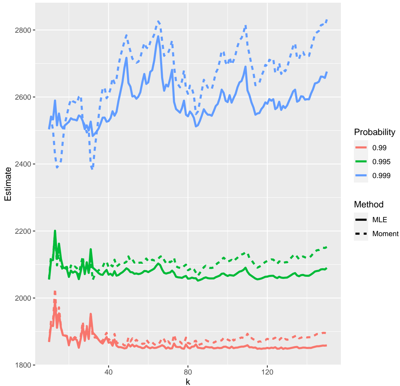
Estimates of high quantiles--22-12-2020
