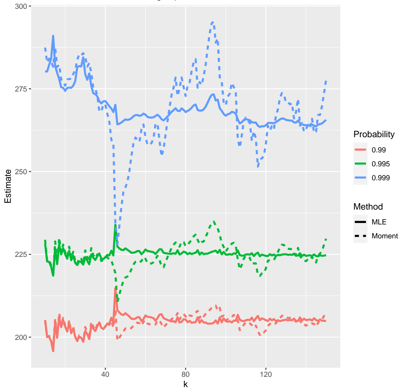
Estimates of high quantiles--22-06-2021
