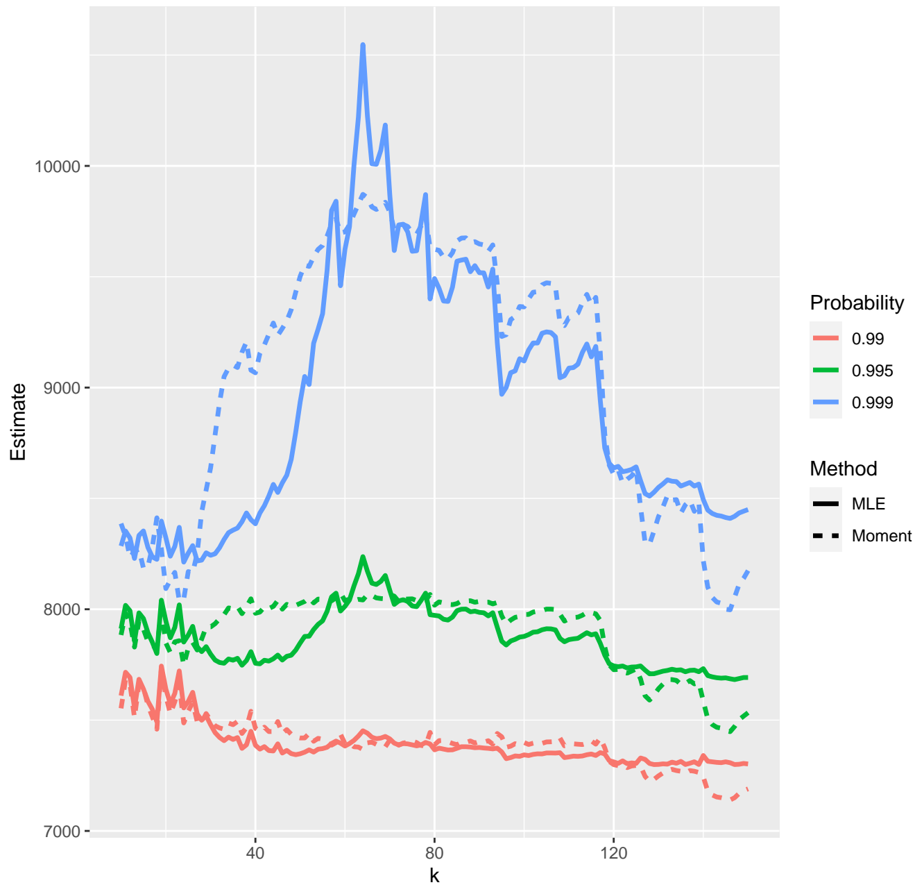
Estimates of high quantiles--22-02-2022
