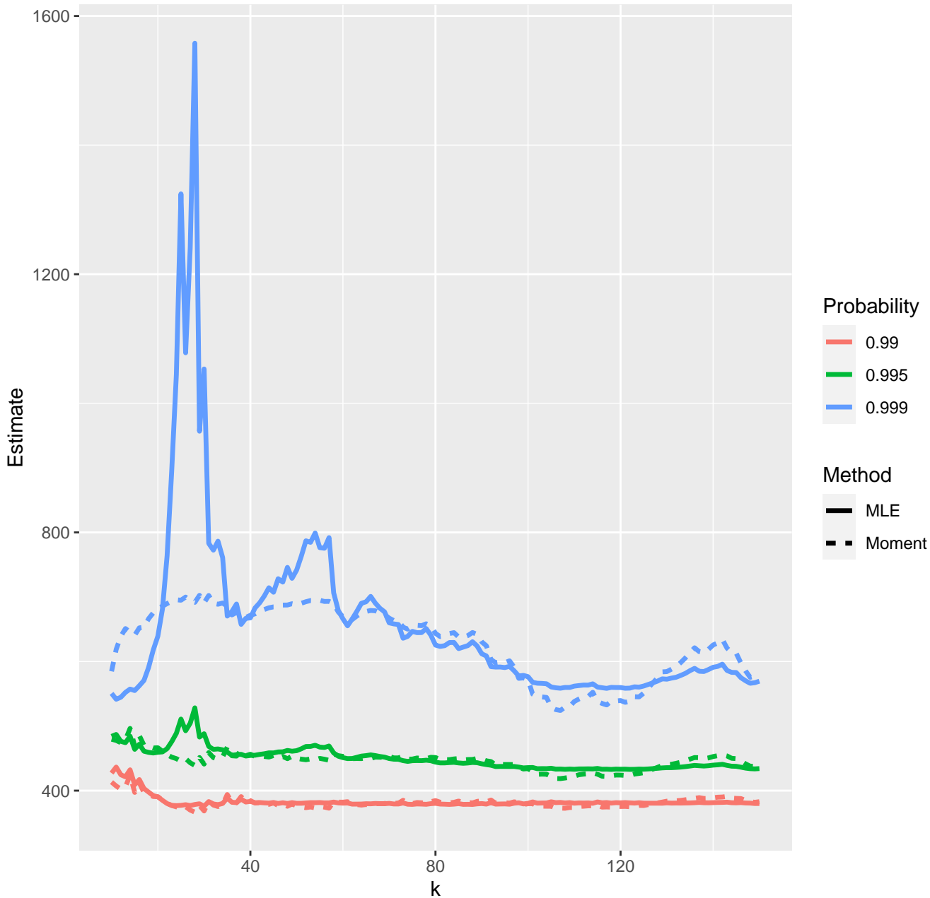
Estimates of high quantiles--21-09-2021
