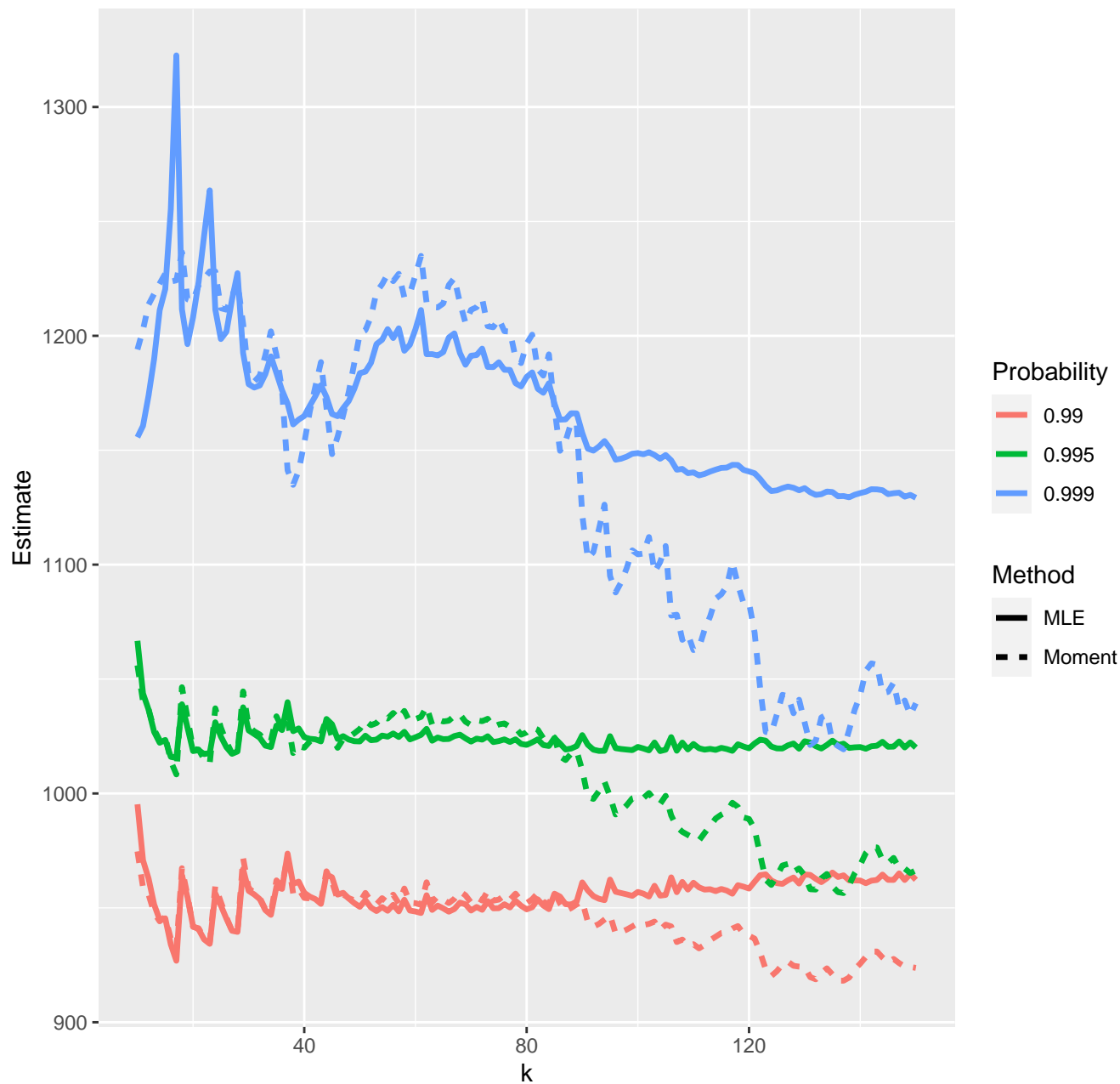
Estimates of high quantiles--20-10-2020
