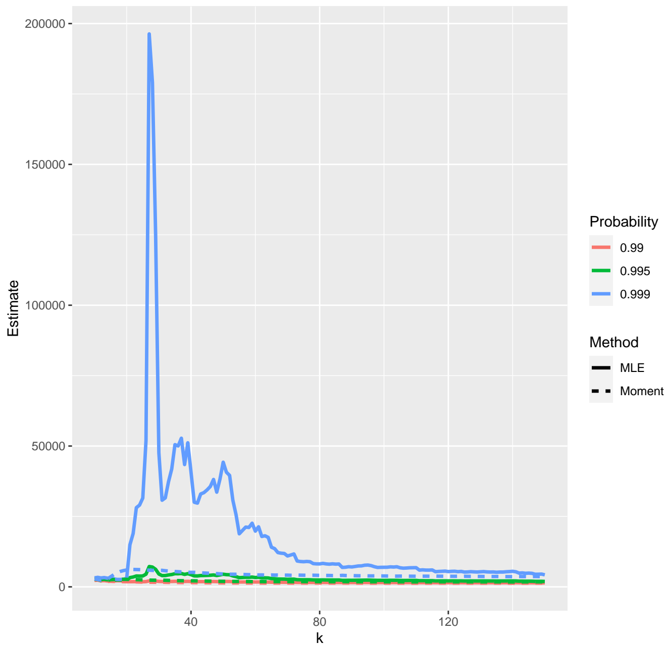
Estimates of high quantiles--19-04-2022
