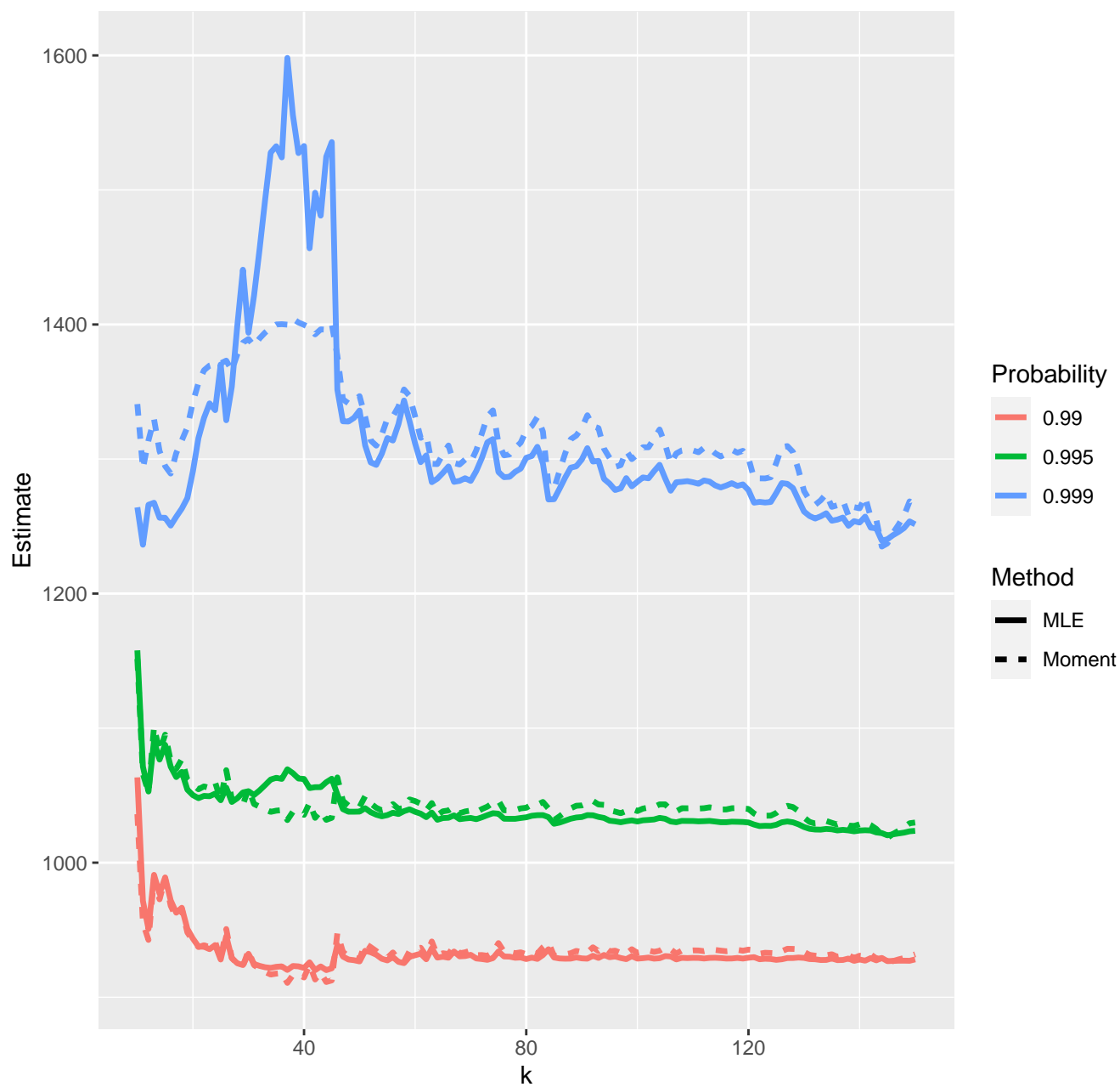
Estimates of high quantiles--18-05-2021
