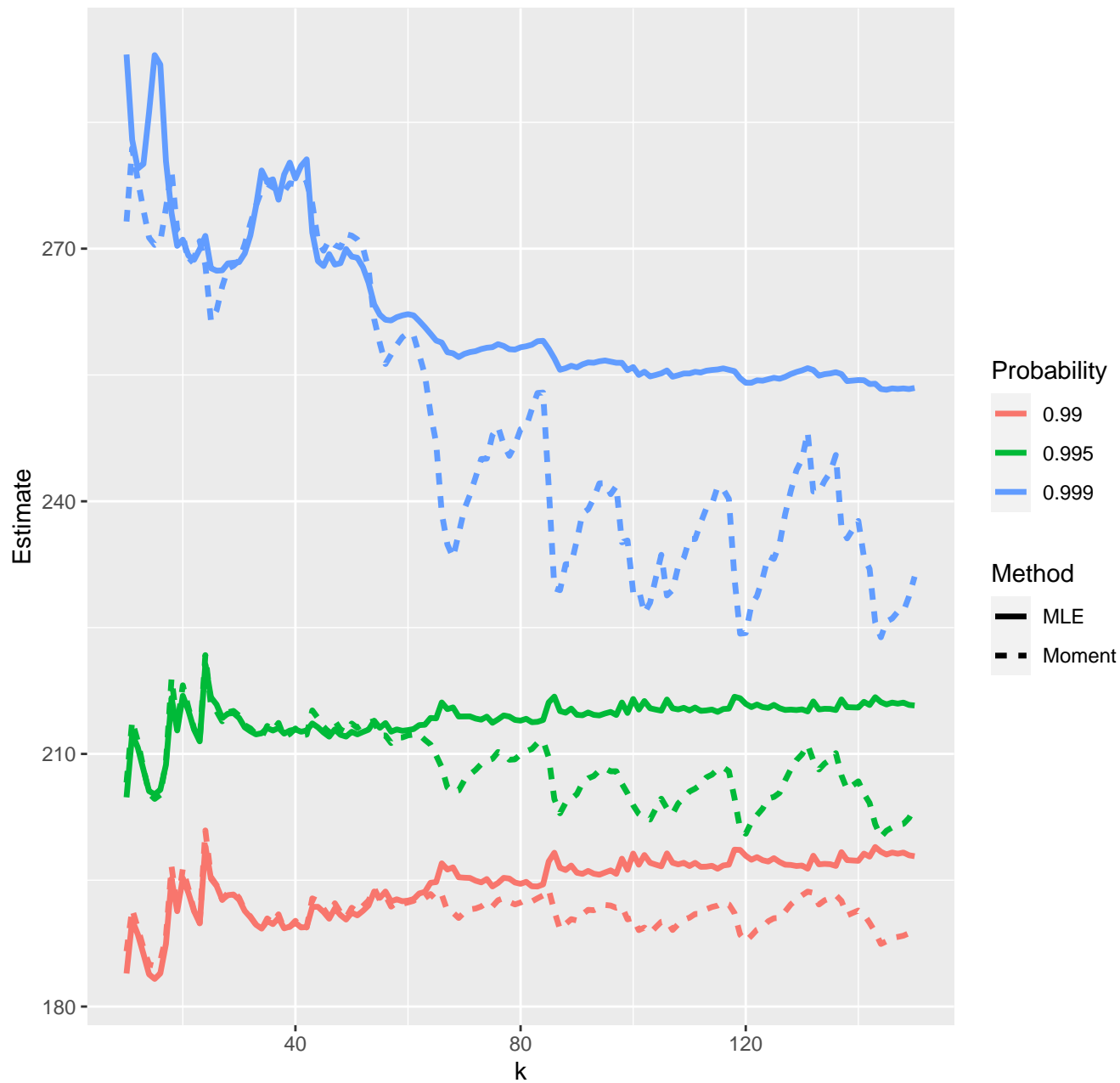
Estimates of high quantiles--17-05-2022
