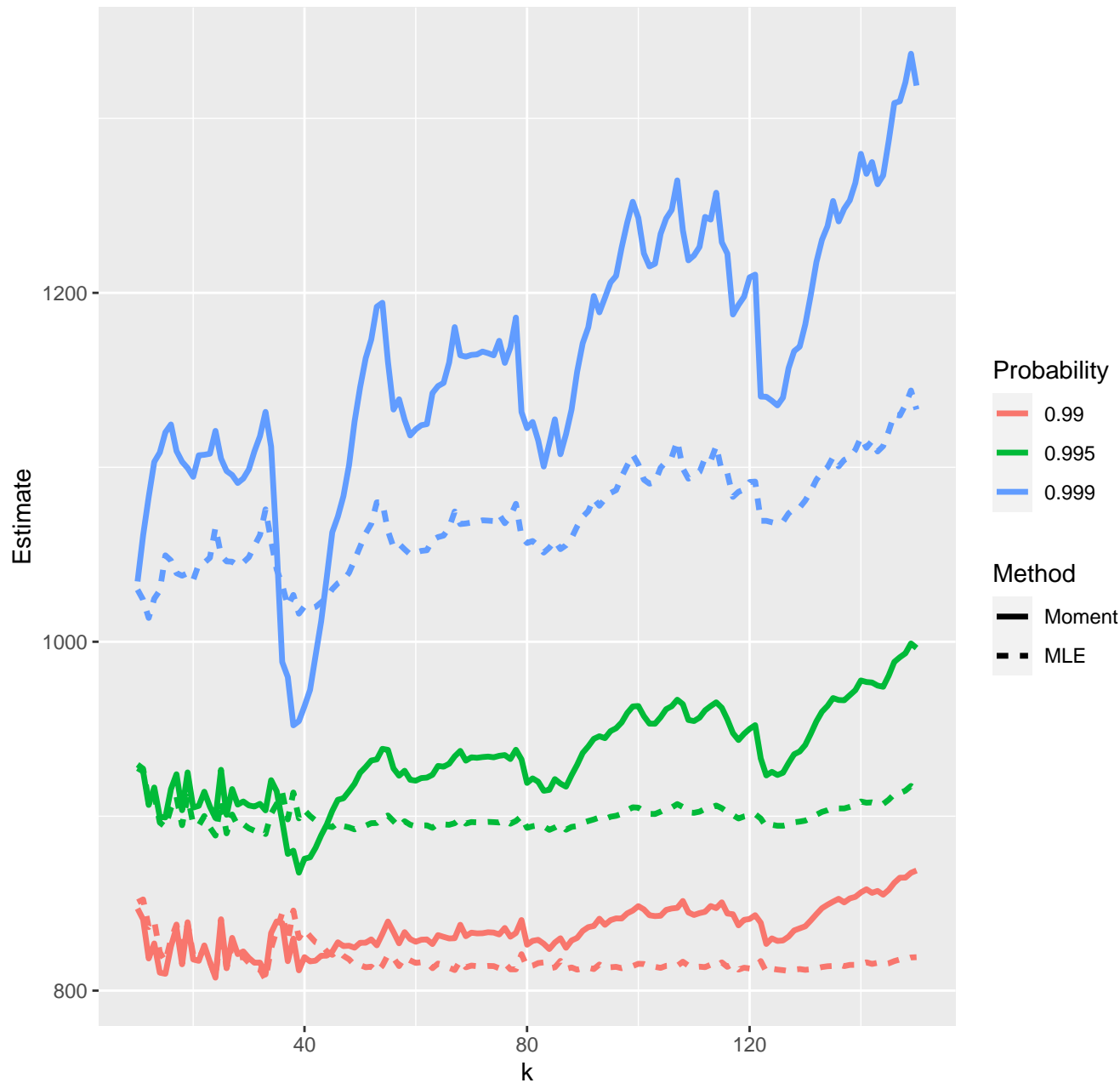
Estimates of high quantiles--15-06-2020
