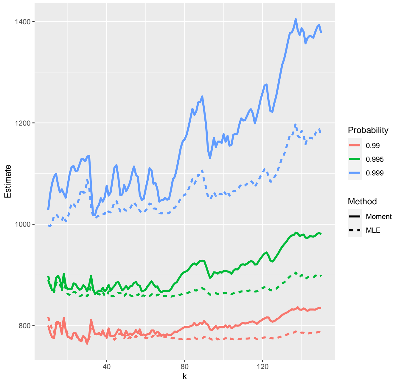
Estimates of high quantiles--15-05-2020
