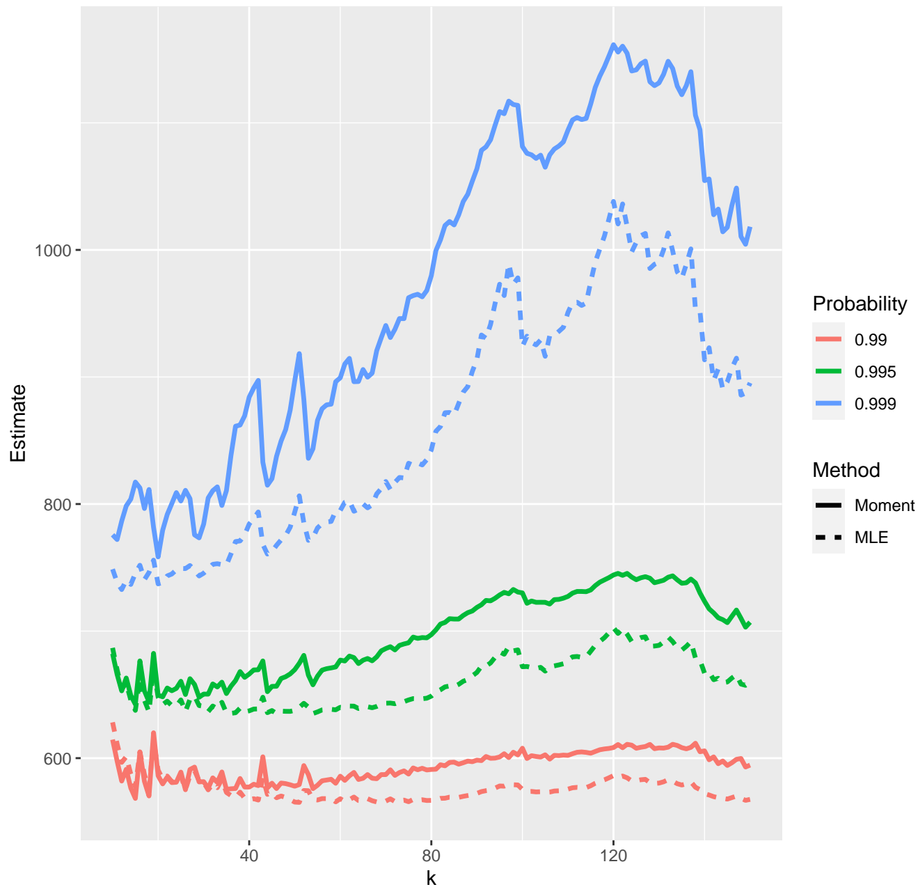
Estimates of high quantiles--14-04-2020
