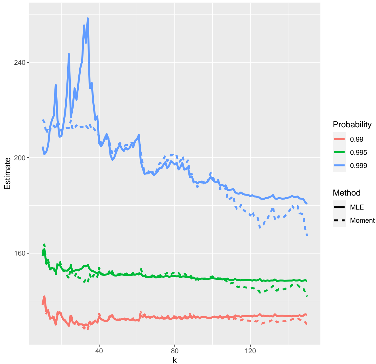
Estimates of high quantiles--13-12-2022
