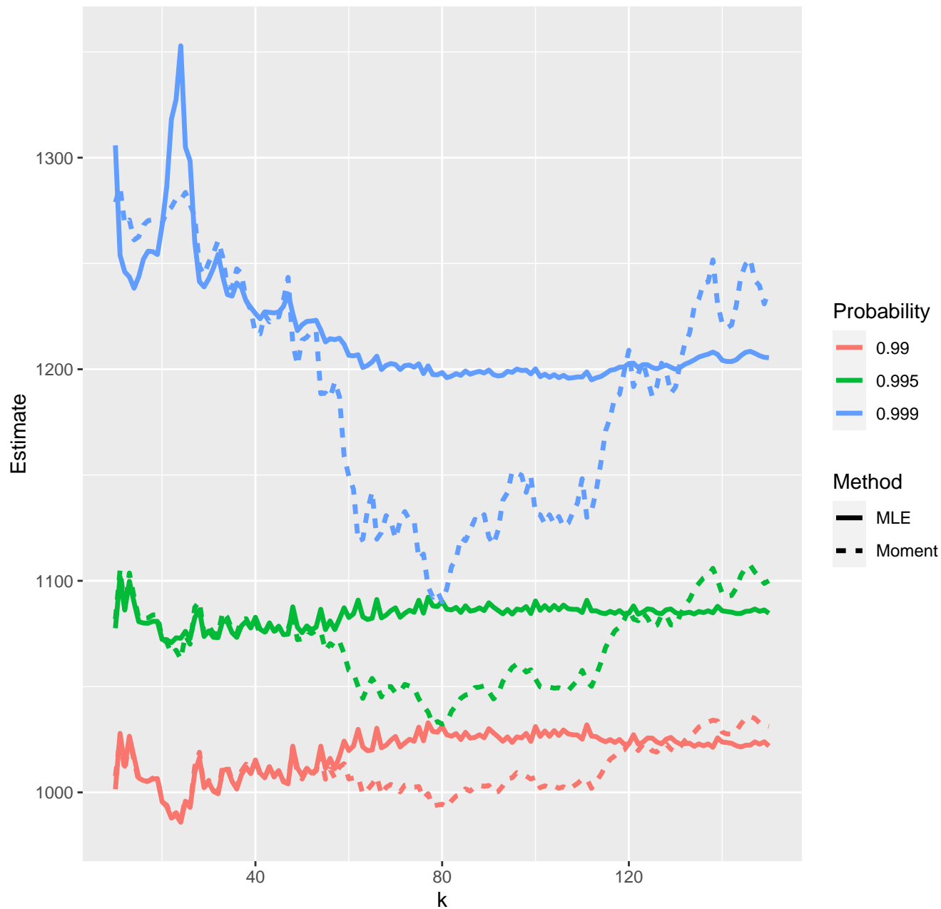
Estimates of high quantiles--11-05-2021
