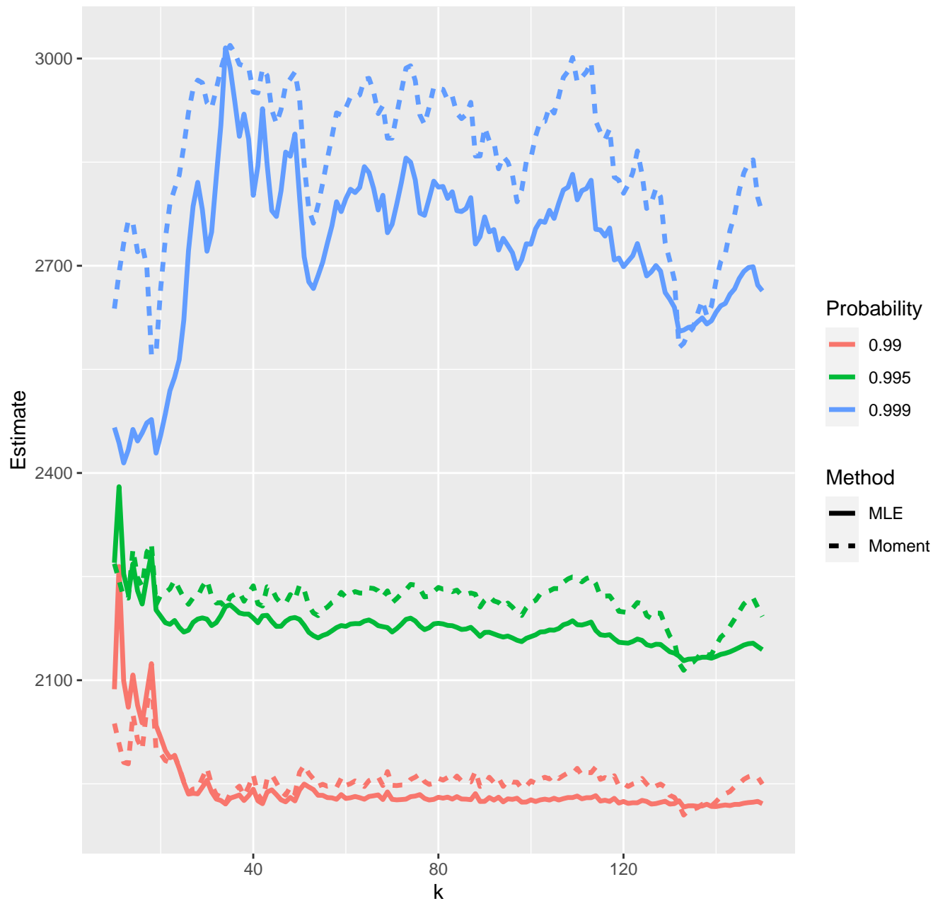
Estimates of high quantiles--10-11-2021
