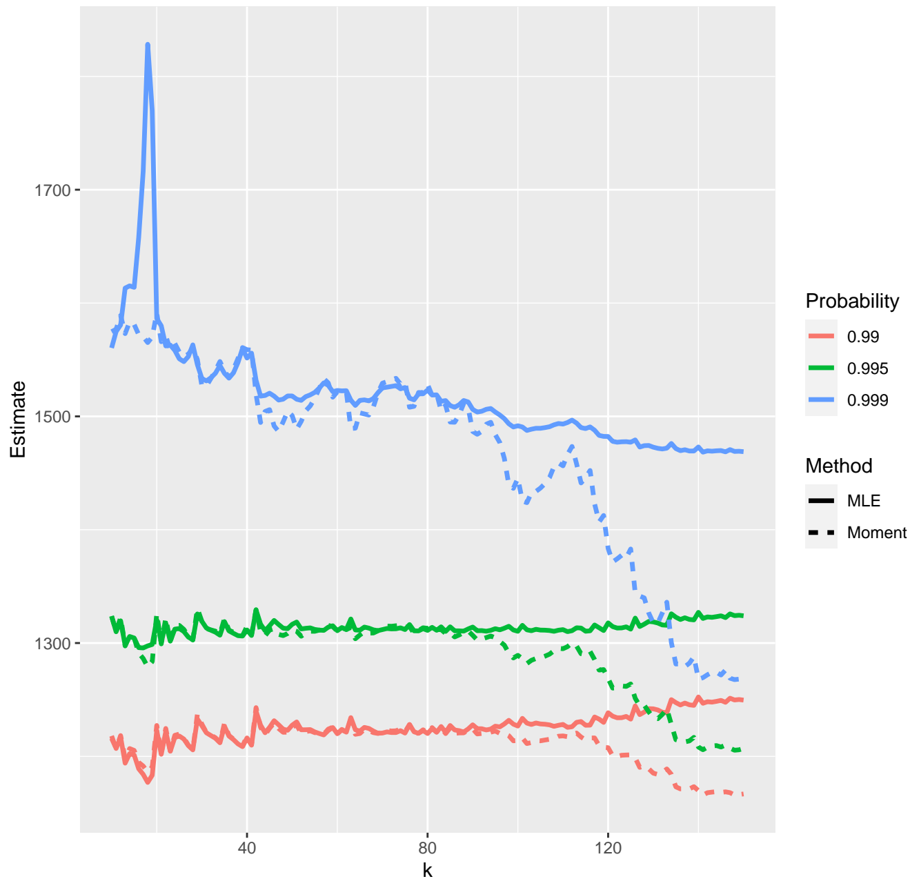
Estimates of high quantiles--10-11-2020
