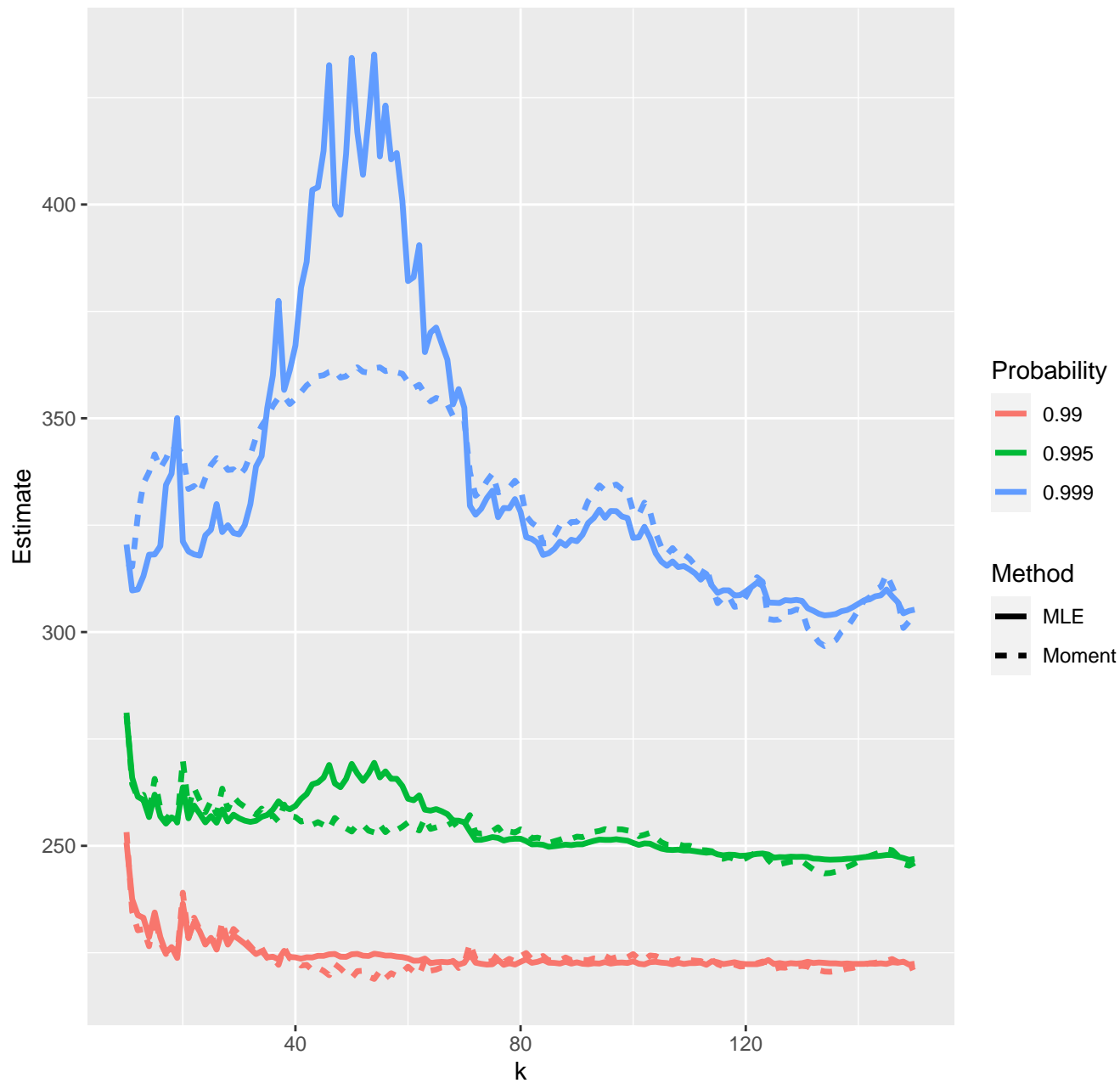
Estimates of high quantiles--10-05-2022
