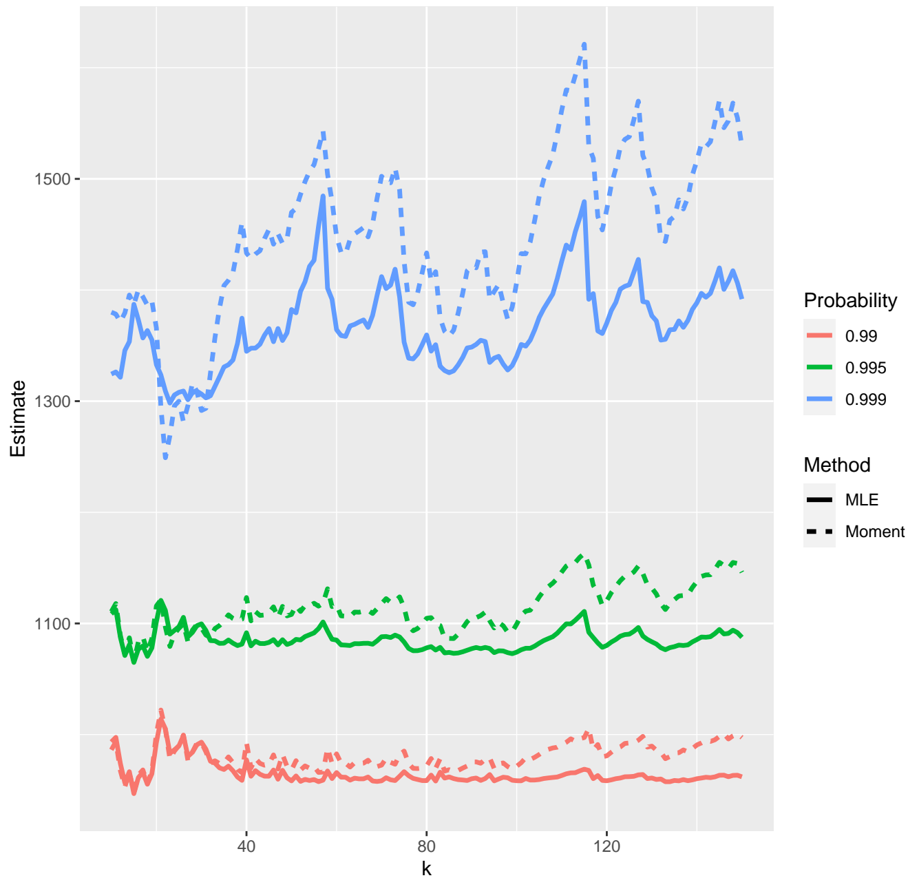
Estimates of high quantiles--09-03-2021
