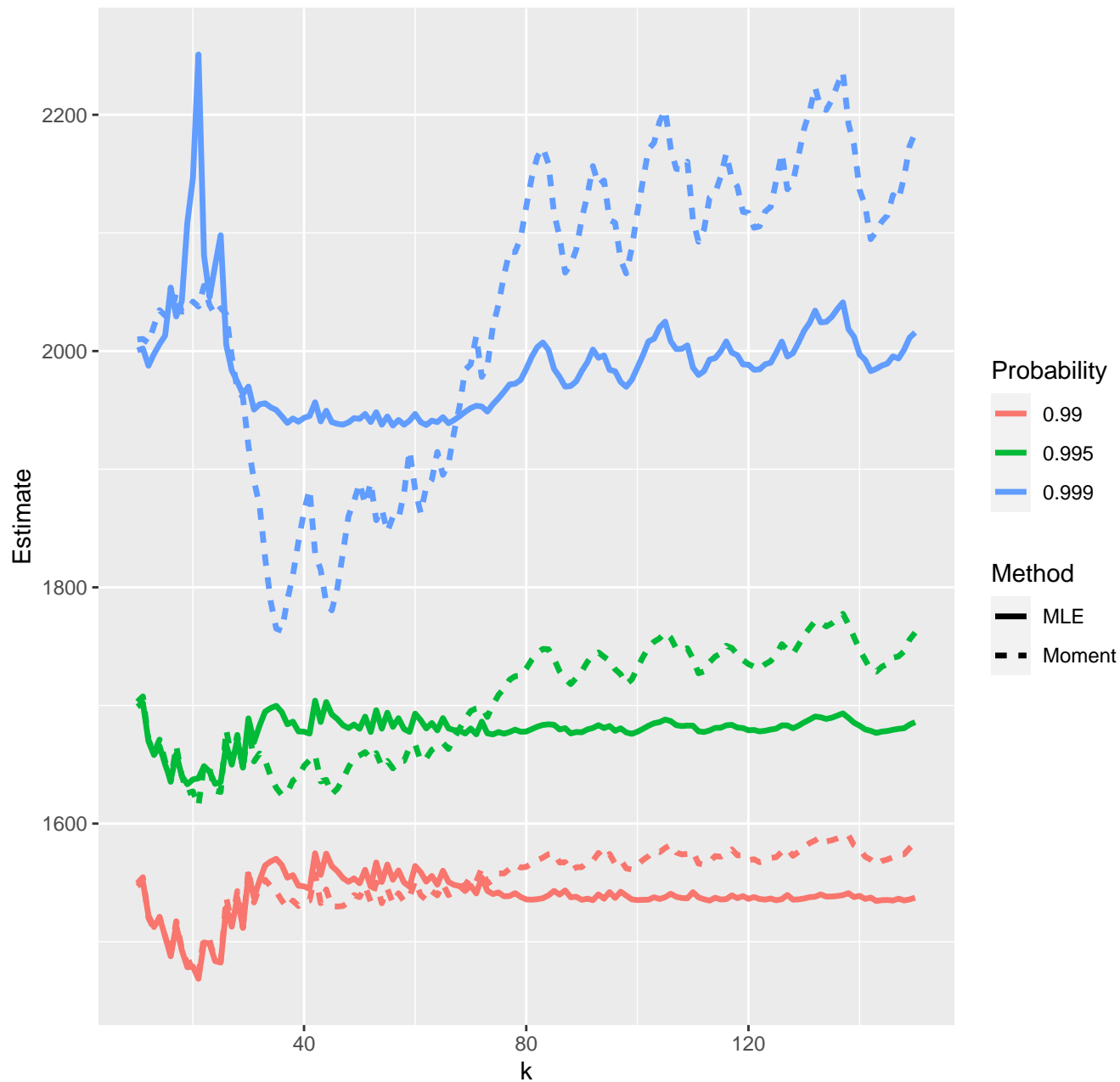
Estimates of high quantiles--06-01-2021
