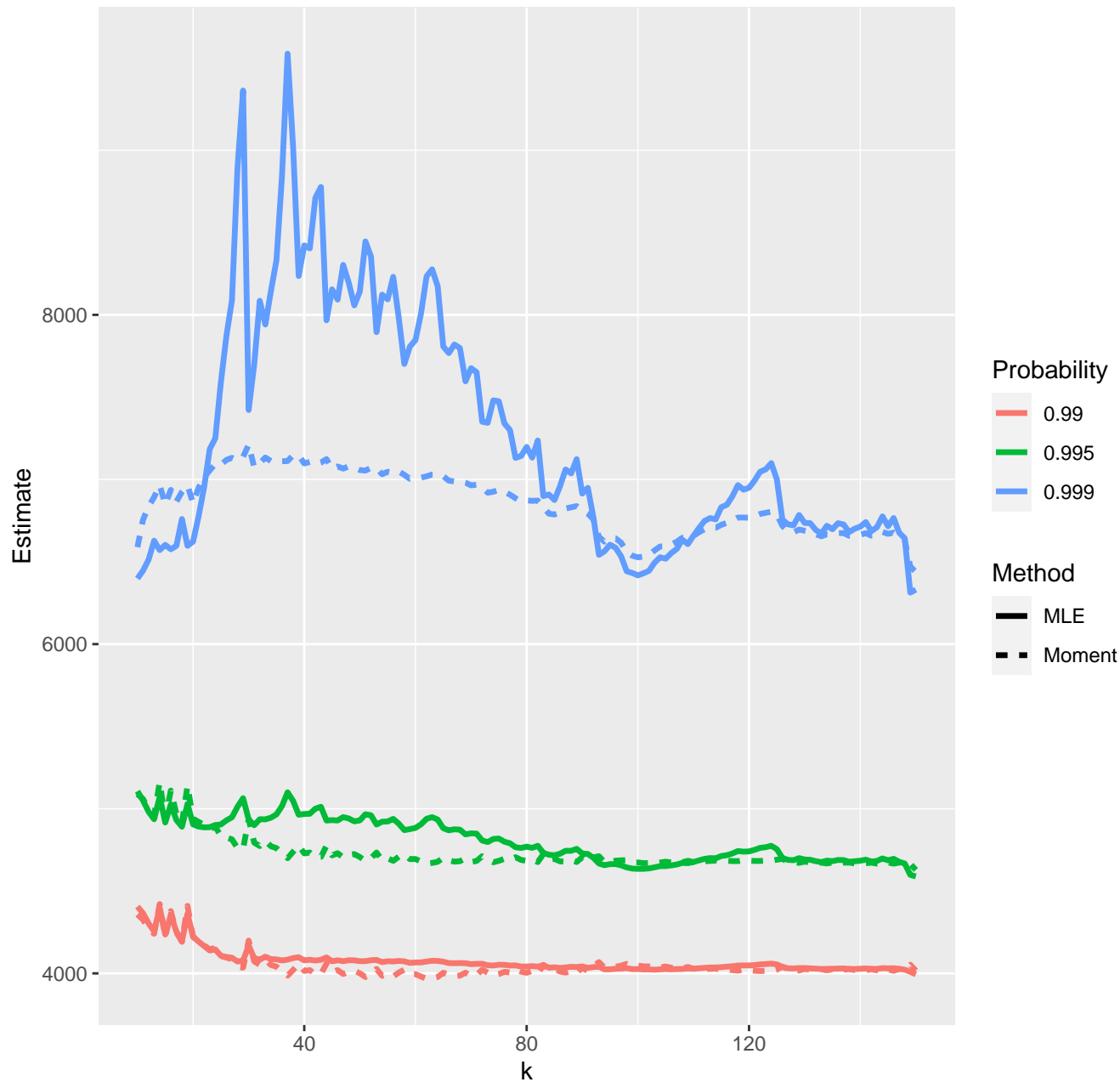
Estimates of high quantiles--05-04-2022
