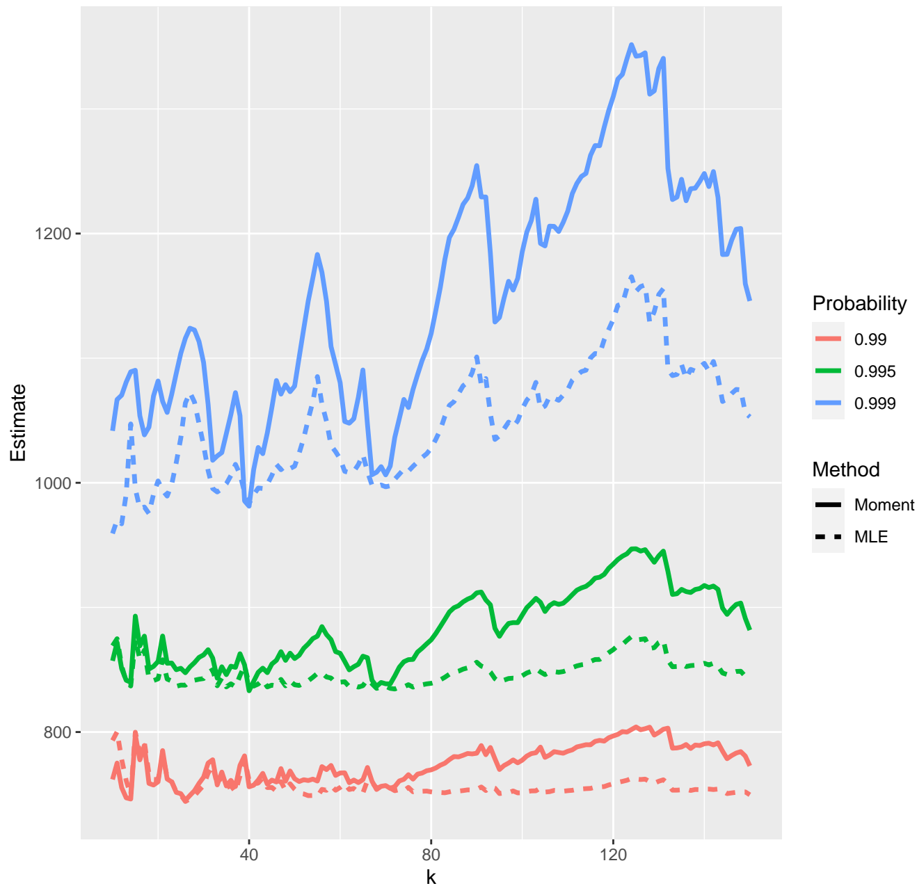
Estimates of high quantiles--04-05-2020
