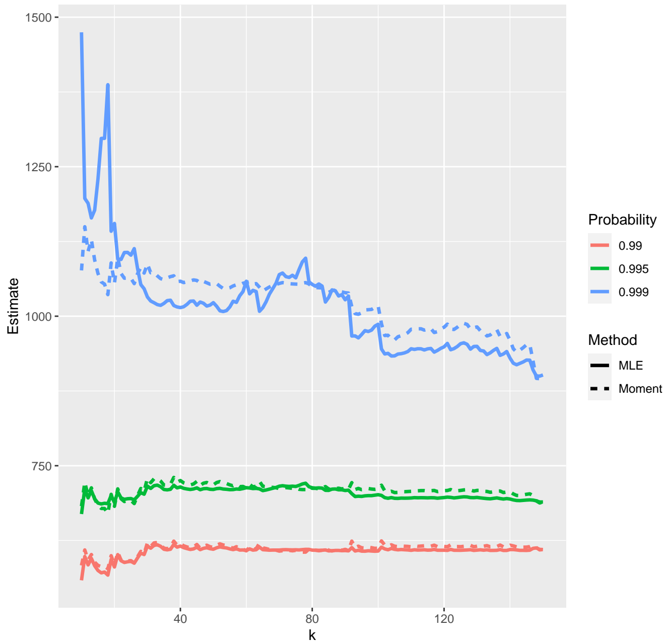
Estimates of high quantiles--03-08-2021
