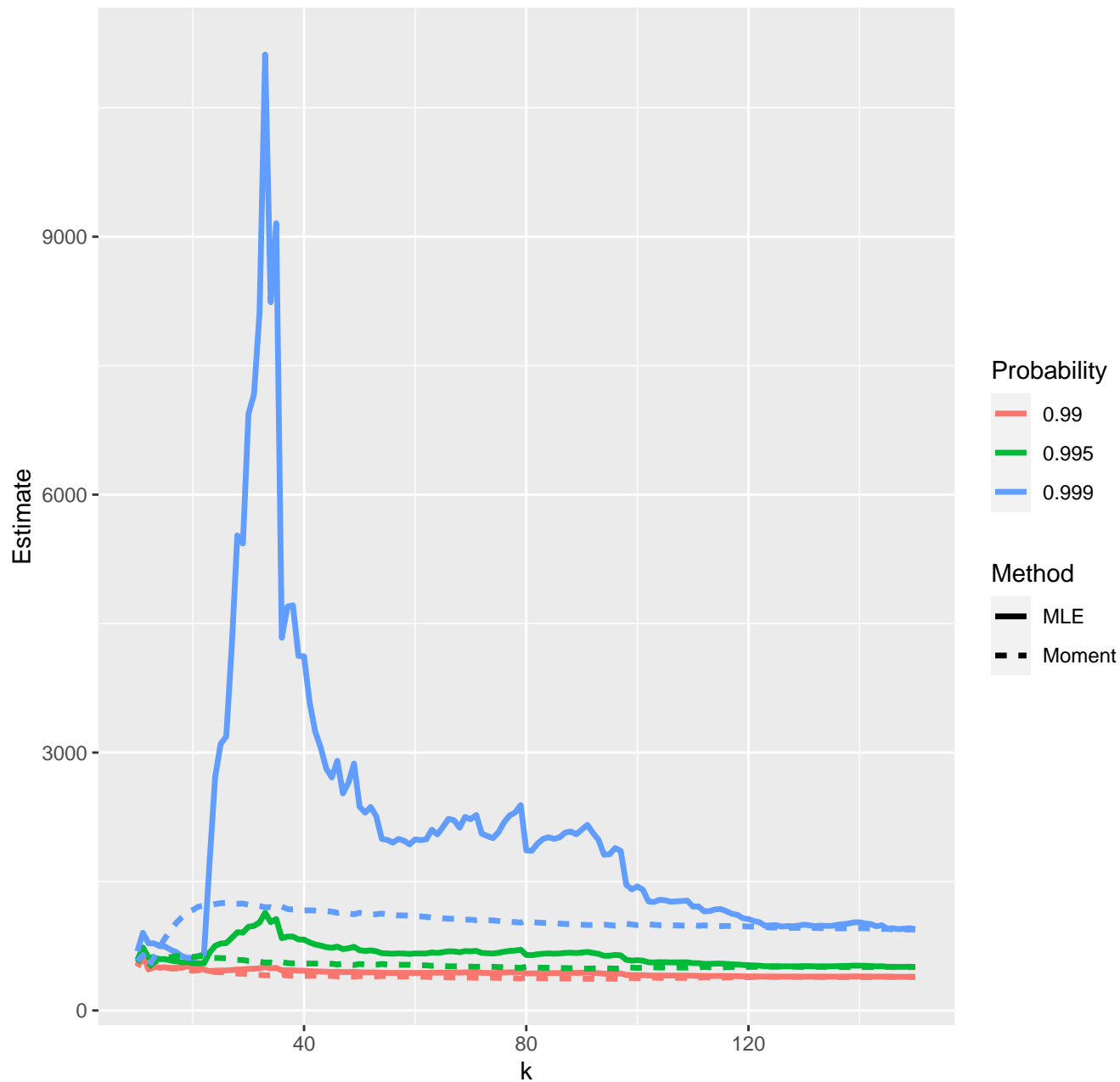
Estimates of high quantiles--03-05-2022
