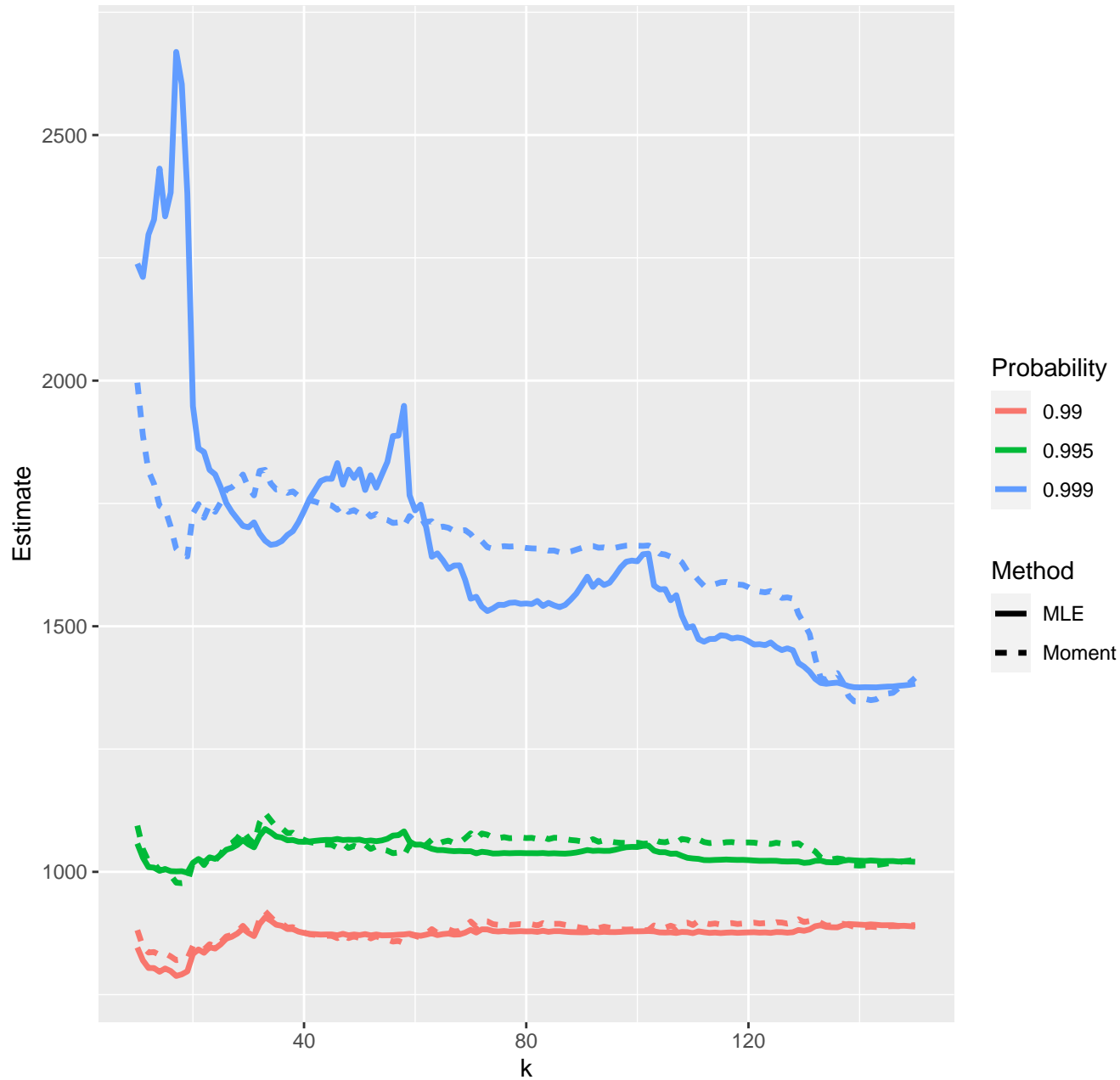
Estimates of high quantiles--02-12-2020
