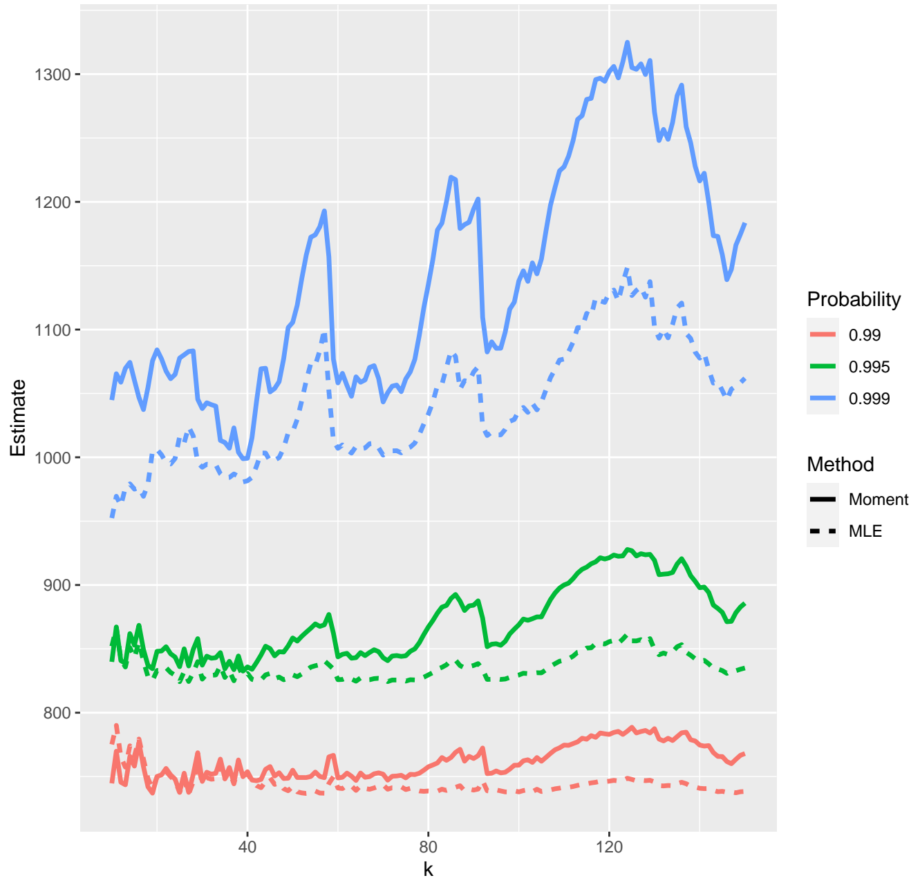
Estimates of high quantiles--01-05-2020
