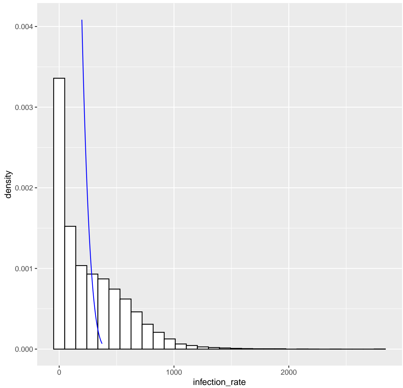
Fitted tail density GPD( 197.6 , 55.18 , -0.2 ), k= 80 -- 31-08-2021
