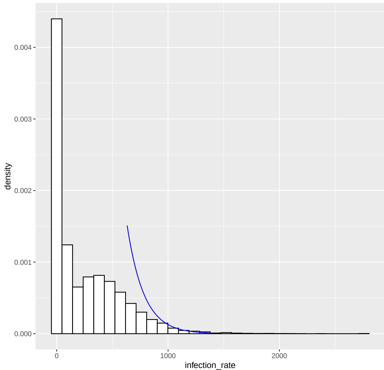
Fitted tail density GPD( 632.6 , 149.12 , -0.01 ), k= 80 -- 30-03-2021
