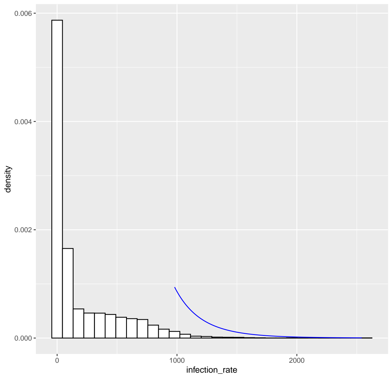
Fitted tail density GPD( 980.1 , 239.56 , 0.1 ), k= 80 -- 29-12-2020
