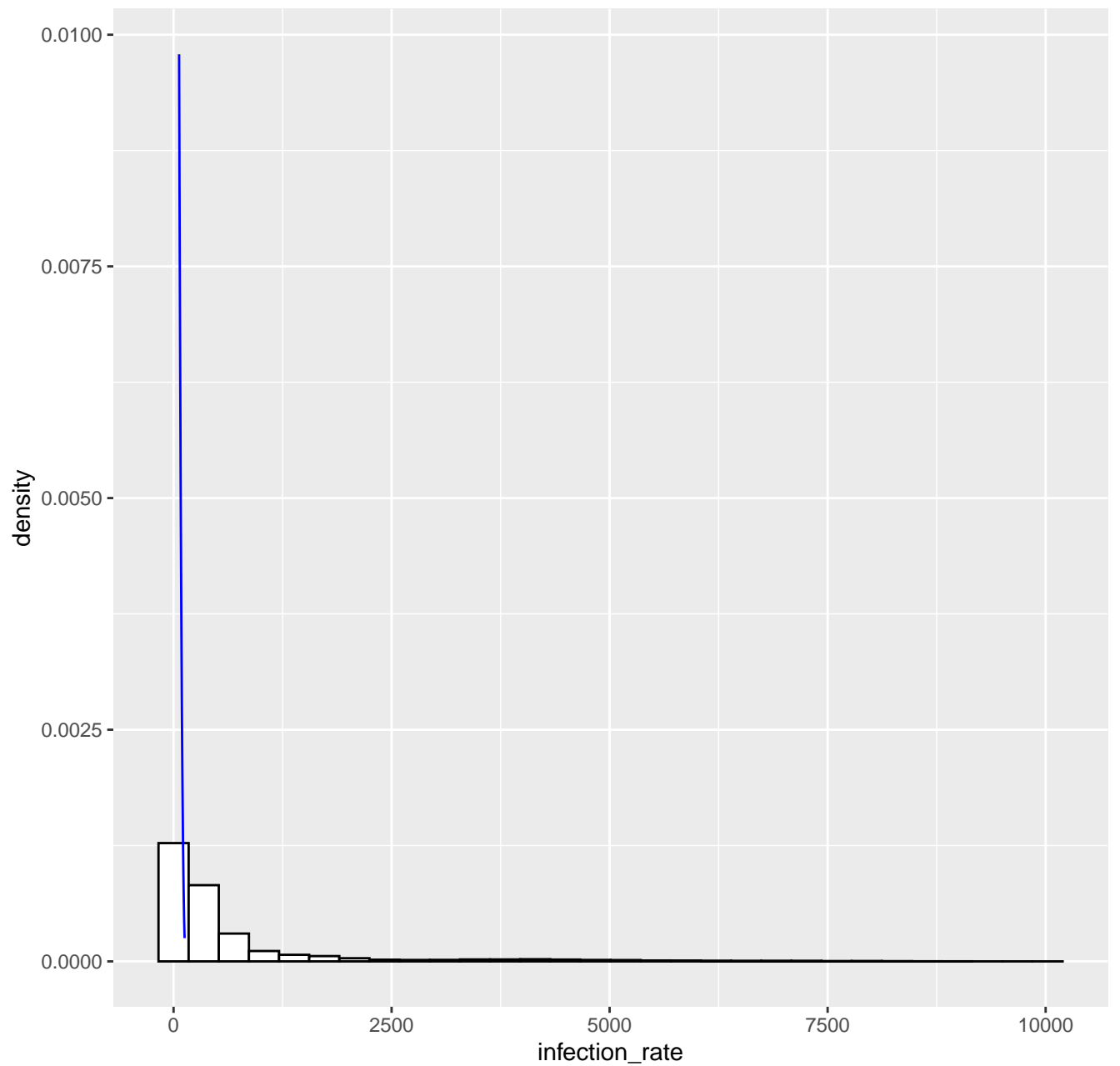
Fitted tail density GPD( 63.3 , 23.02 , -0.27 ), k= 80 -- 29-11-2022
