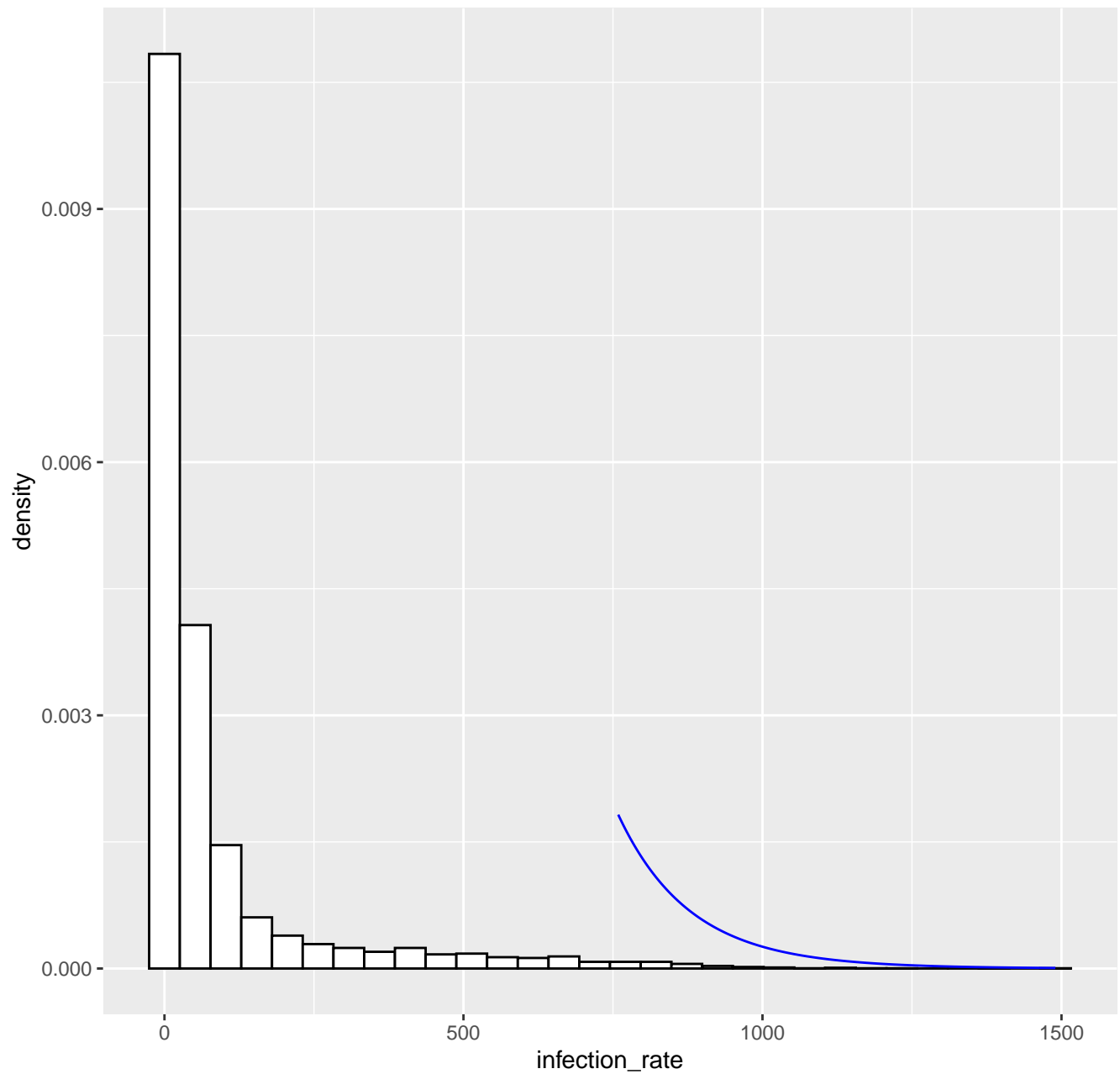
Fitted tail density GPD( 758.8 , 123.61 , 0.03 ), k= 80 -- 29-10-2020
