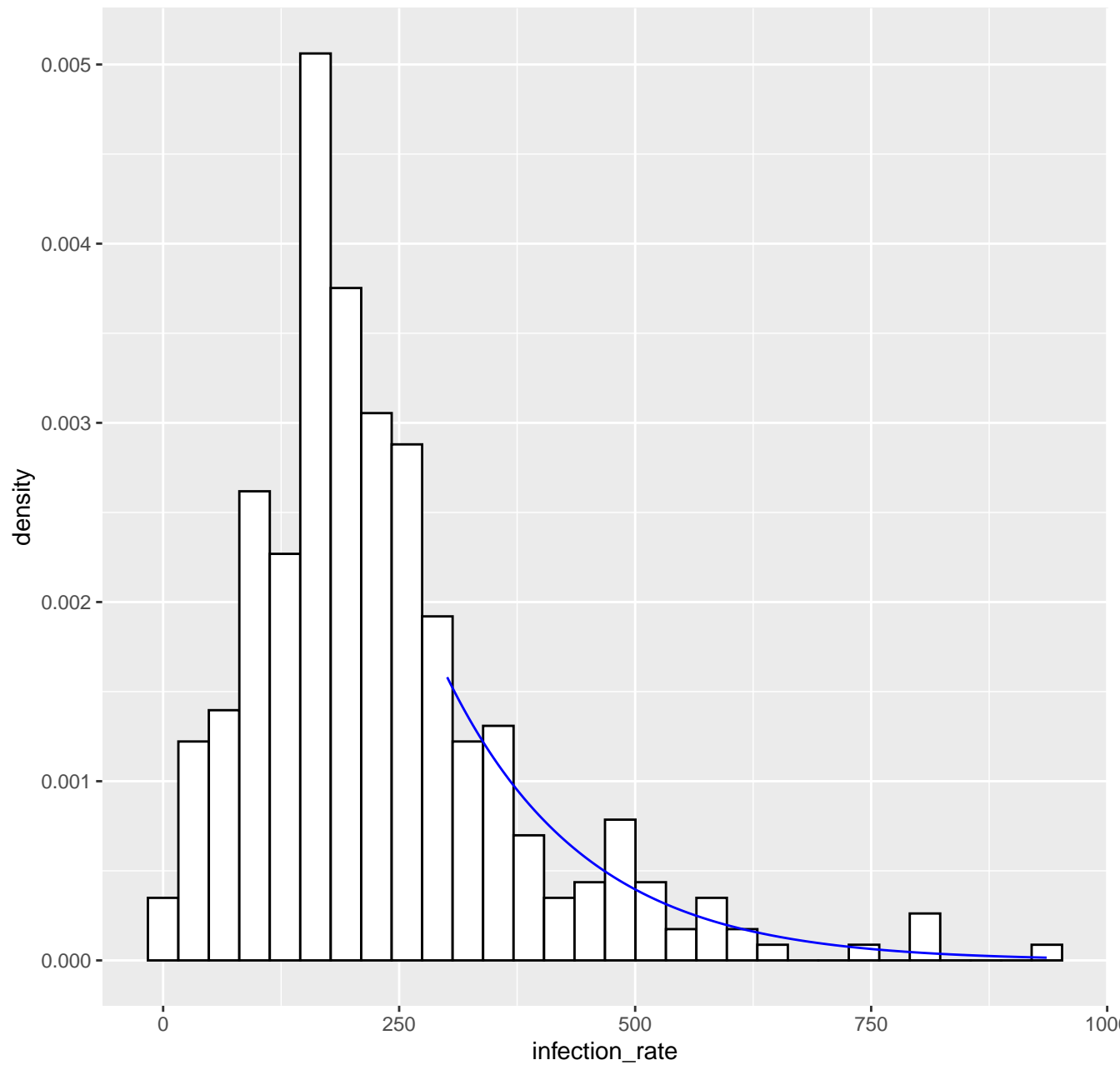
Fitted tail density GPD( 300.9 , 142.58 , -0.03 ), k= 80 -- 29-04-2020
