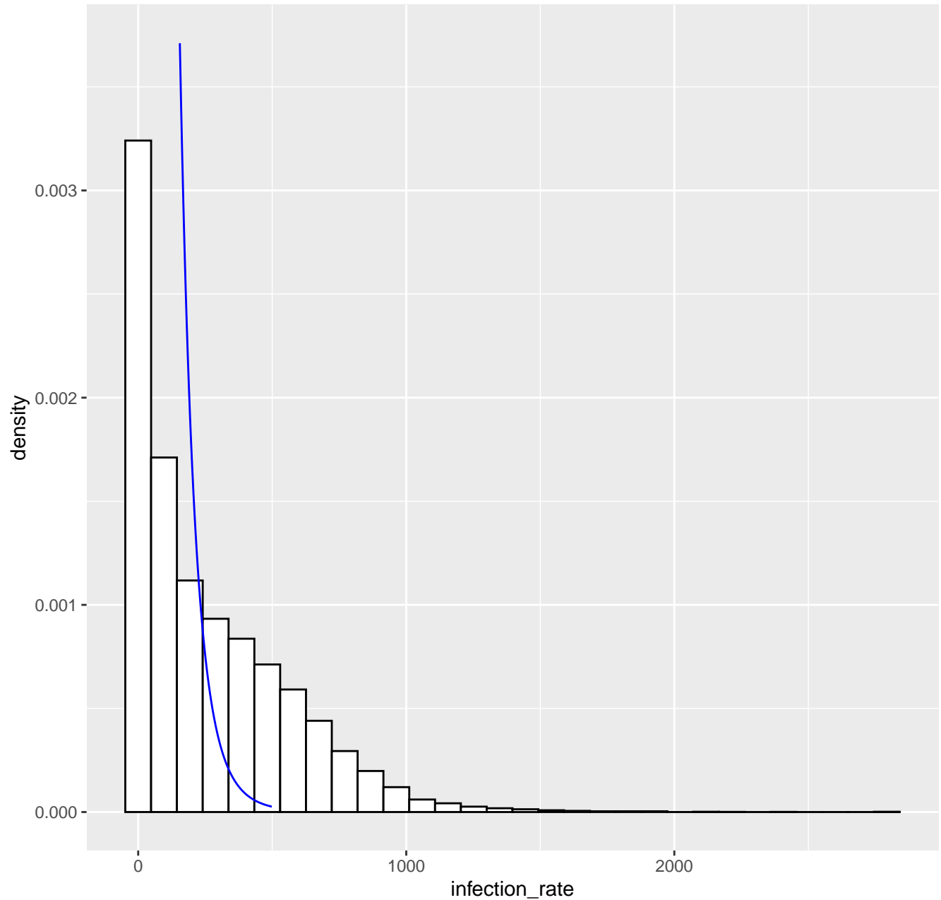
Fitted tail density GPD( 155.4 , 60.73 , 0.09 ), k= 80 -- 28-09-2021
