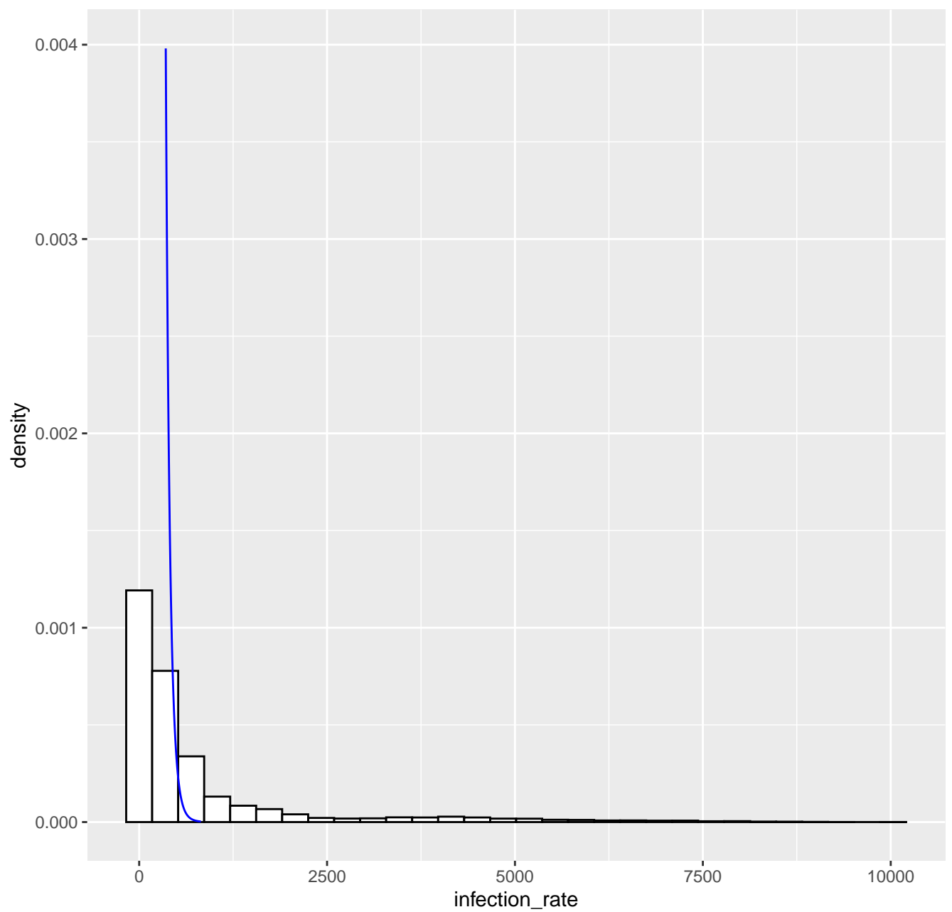
Fitted tail density GPD( 353.7 , 56.61 , 0.05 ), k= 80 -- 28-06-2022
