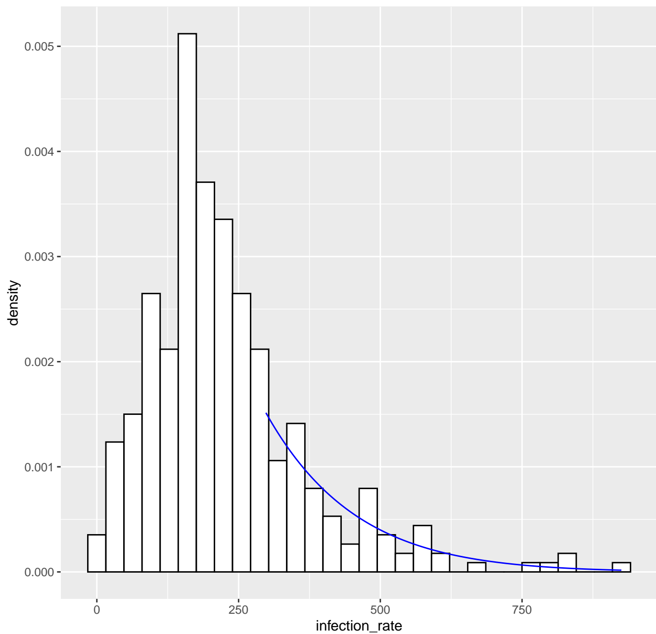
Fitted tail density GPD( 298.2 , 148.85 , -0.05 ), k= 80 -- 28-04-2020
