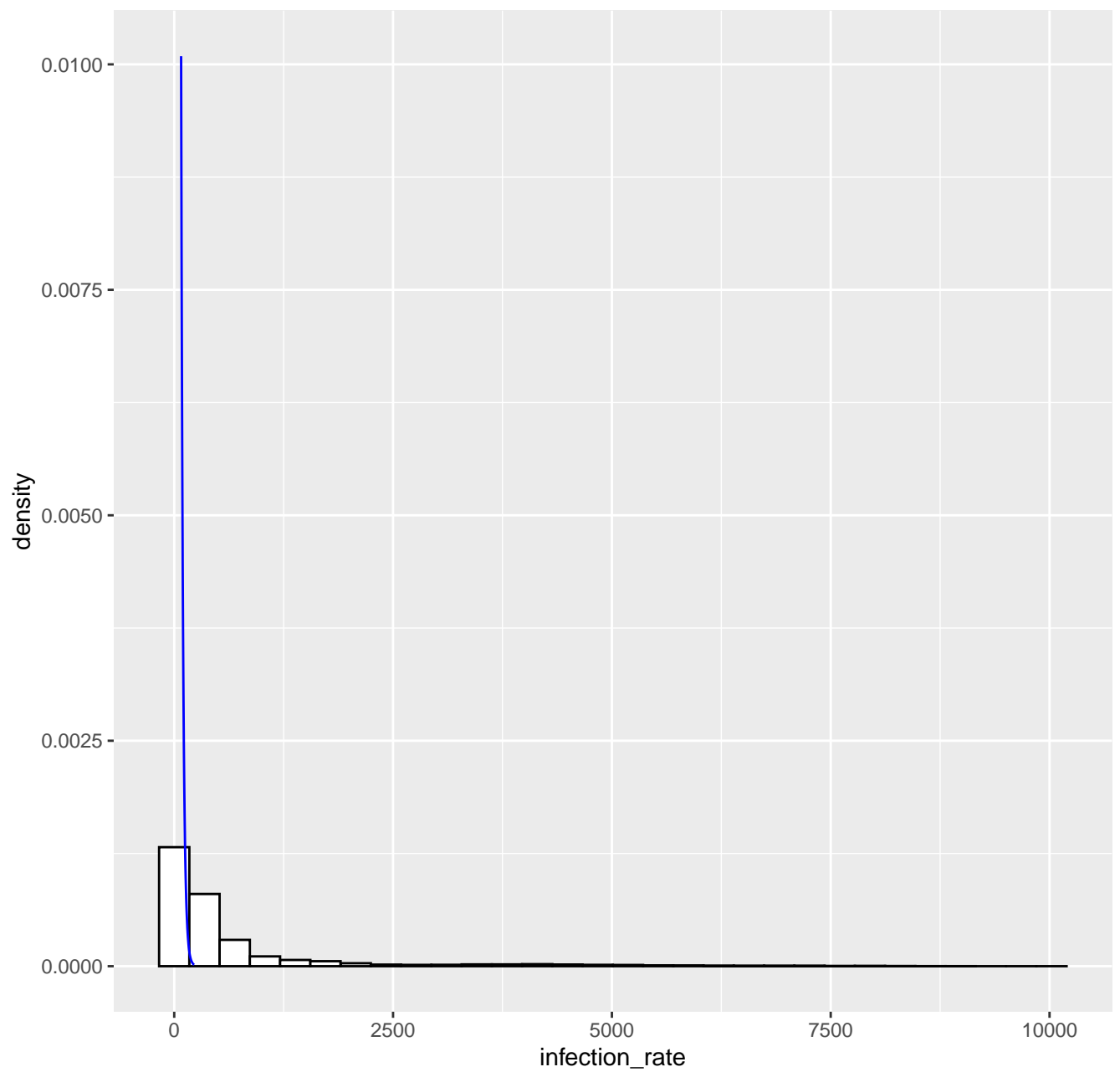
Fitted tail density GPD( 78.6 , 22.33 , 0.01 ), k= 80 -- 27-12-2022
