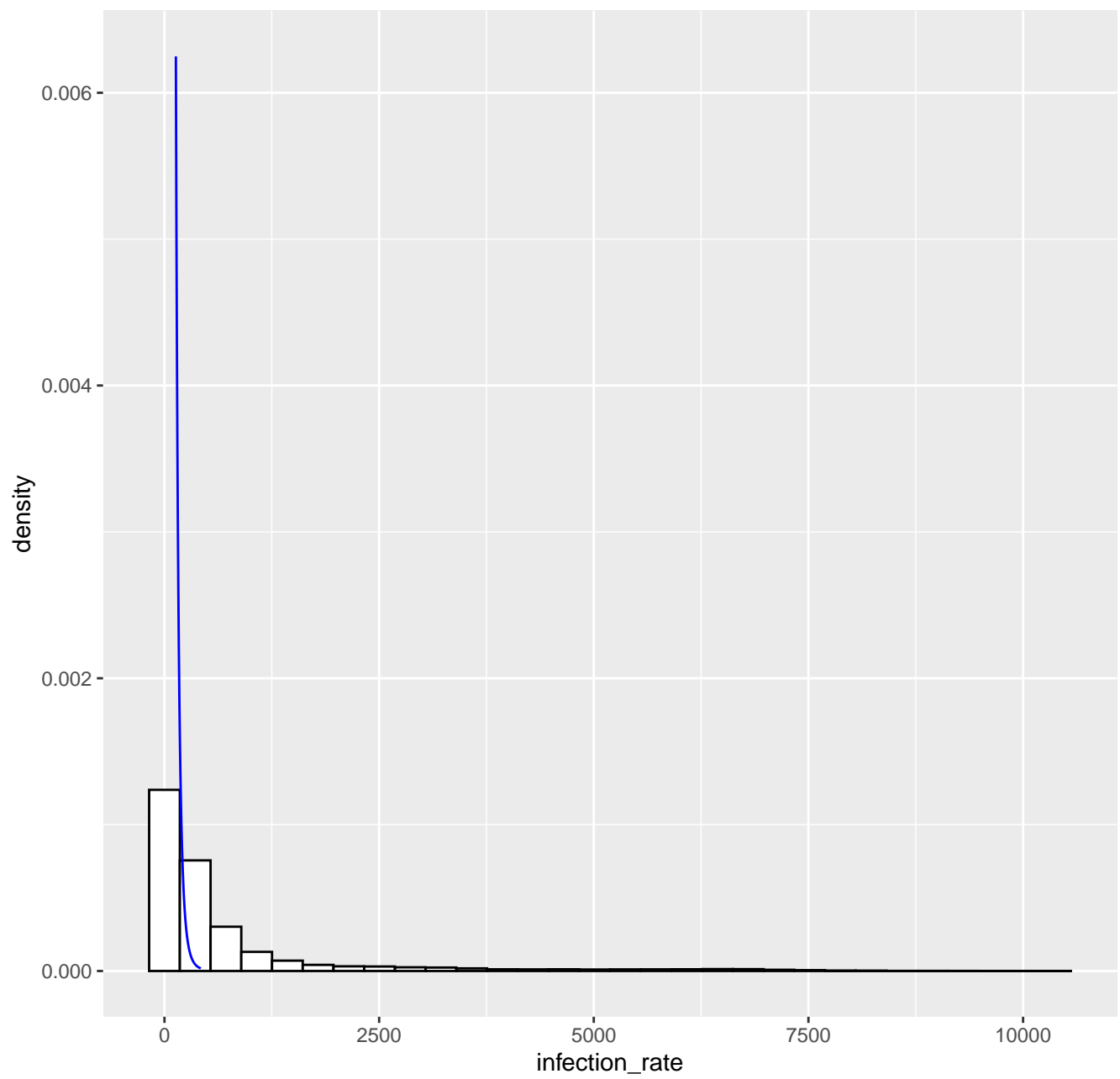
Fitted tail density GPD( 132.8 , 36.07 , 0.18 ), k= 80 -- 27-09-2022
