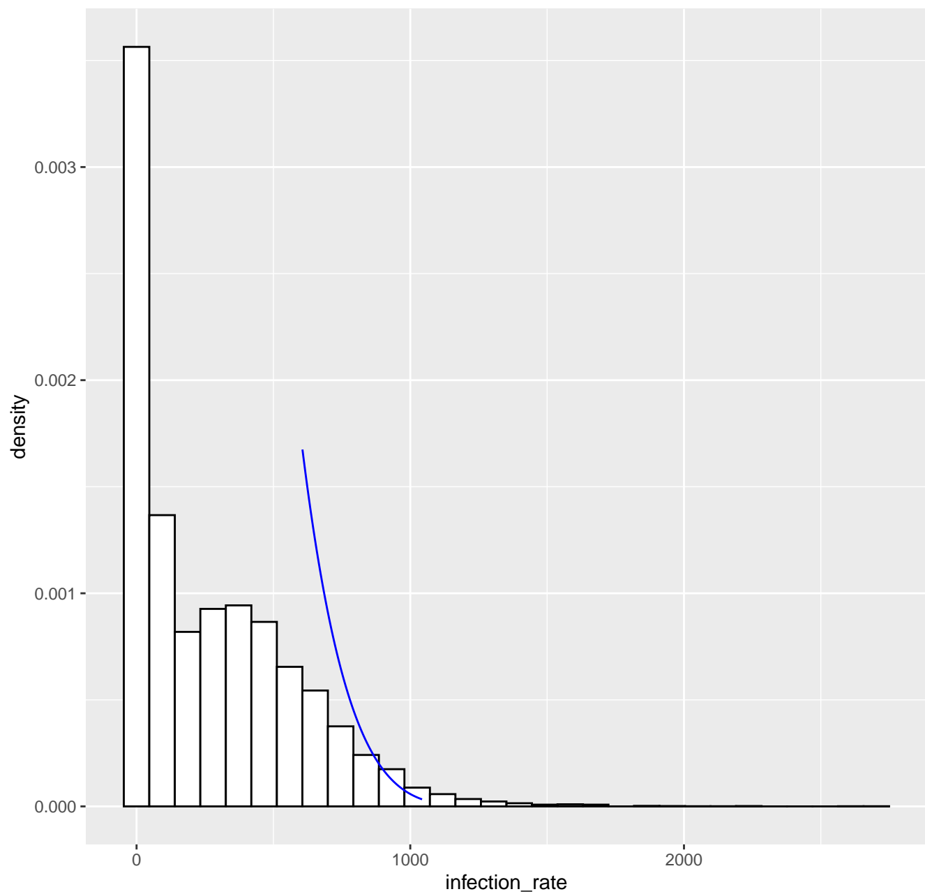
Fitted tail density GPD( 606.1 , 134.56 , -0.17 ), k= 80 -- 27-07-2021
