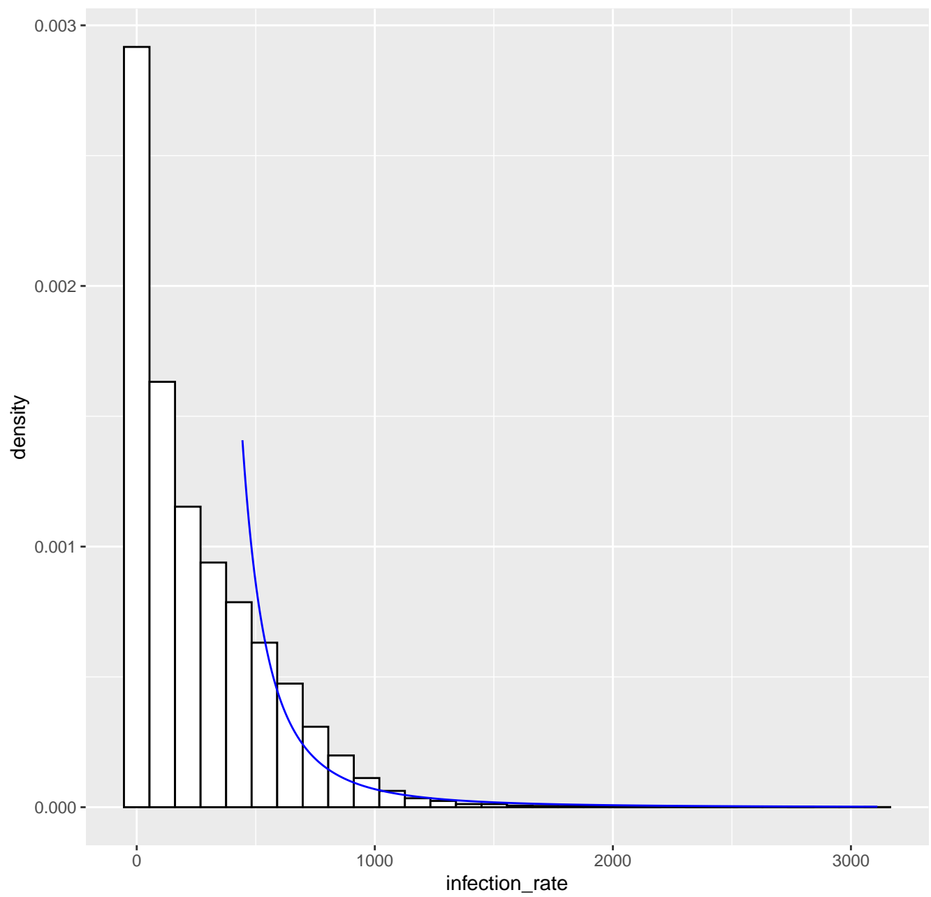
Fitted tail density GPD( 444.1 , 160.05 , 0.55 ), k= 80 -- 26-10-2021
