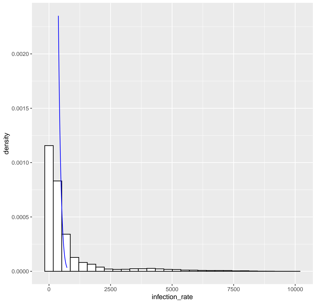
Fitted tail density GPD( 380 , 95.86 , -0.12 ), k= 80 -- 26-07-2022
