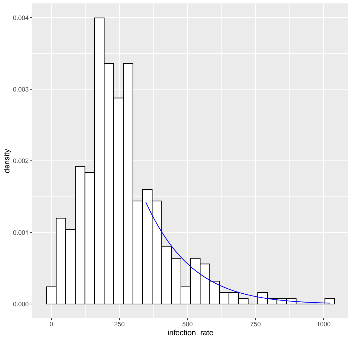
Fitted tail density GPD( 346.9 , 158.41 , -0.07 ), k= 80 -- 26-05-2020
