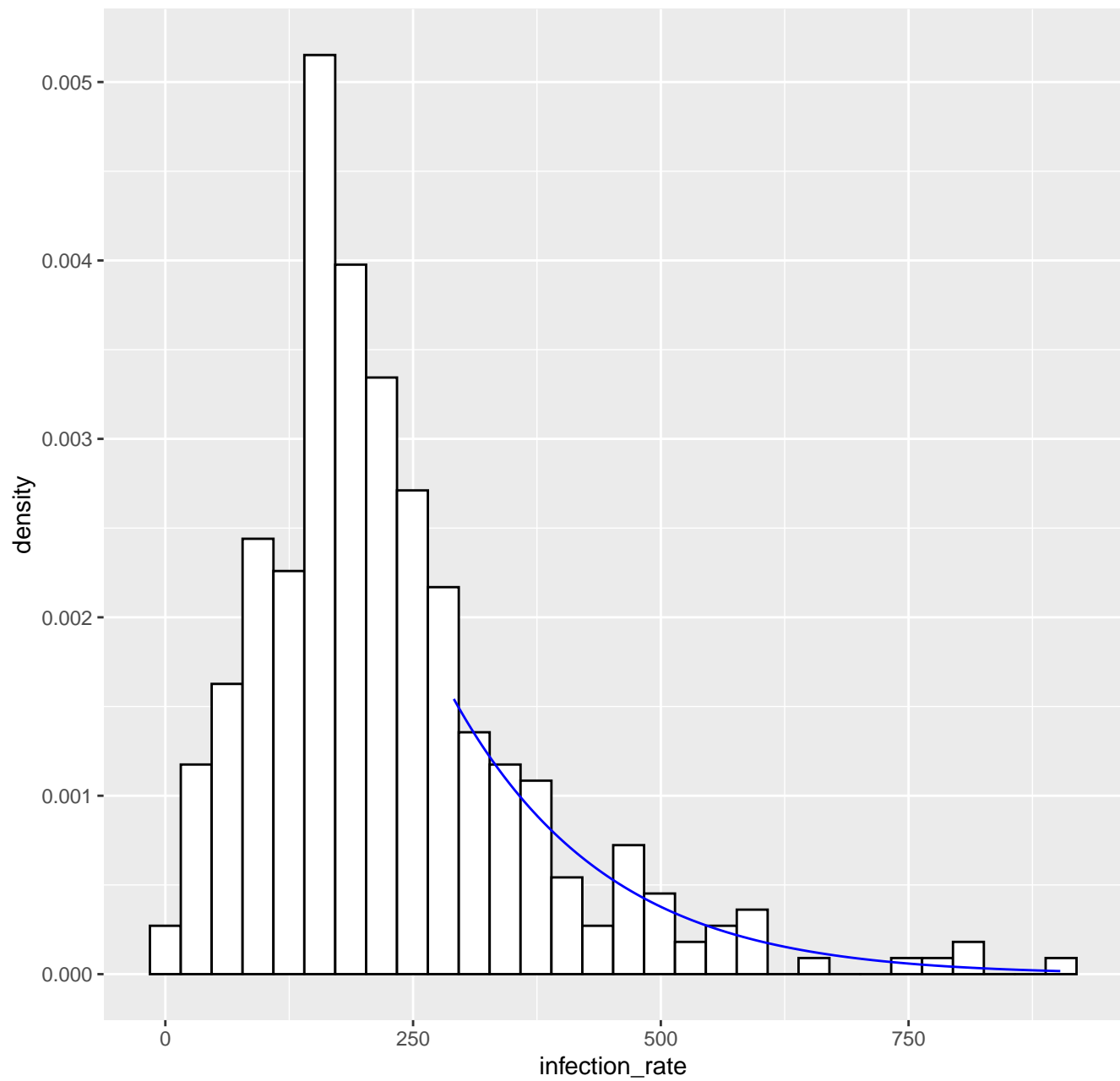
Fitted tail density GPD( 291.1 , 146.12 , -0.06 ), k= 80 -- 26-04-2020
